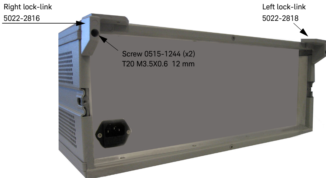
Figure 11 Install Rear Lock-links to the Test Set
