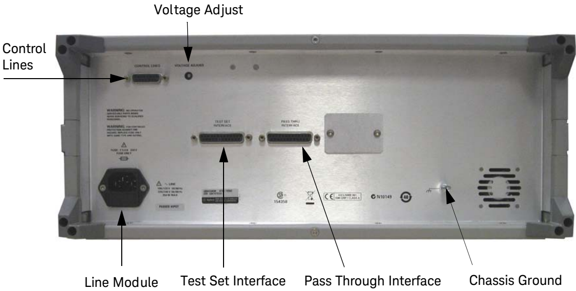
Figure 7 U3022AM06 Rear Panel
