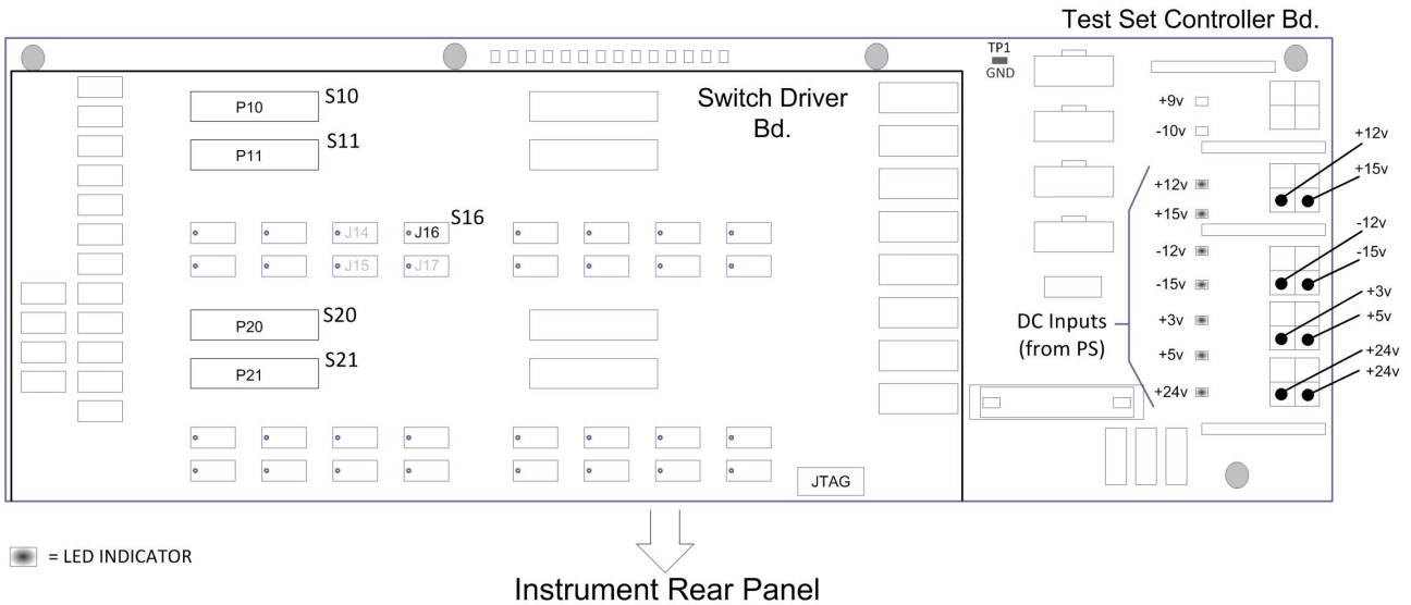
Figure 67 DC Power Status LEDs
