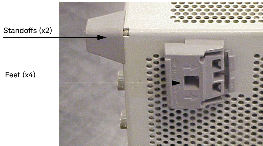
Figure 14 Rear Bottom Feet
