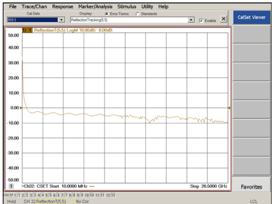
Figure 62 Typical Reflection Tracking with N5242A/B (Ports 1 - 2)
