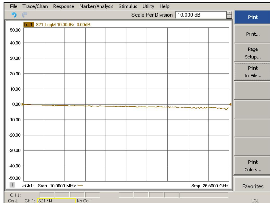
Figure 69 Source IN to Cplr Thru & Rcvr Out to Cplr Path Response
