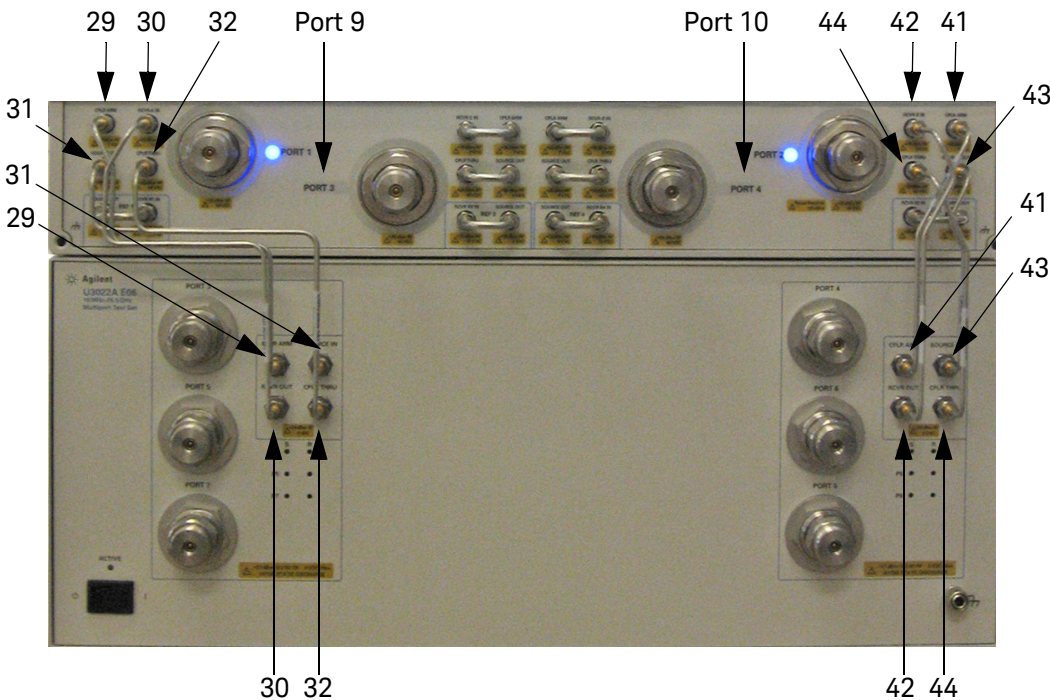
Figure 26 N5242A/B RF Interface Cable Connections
