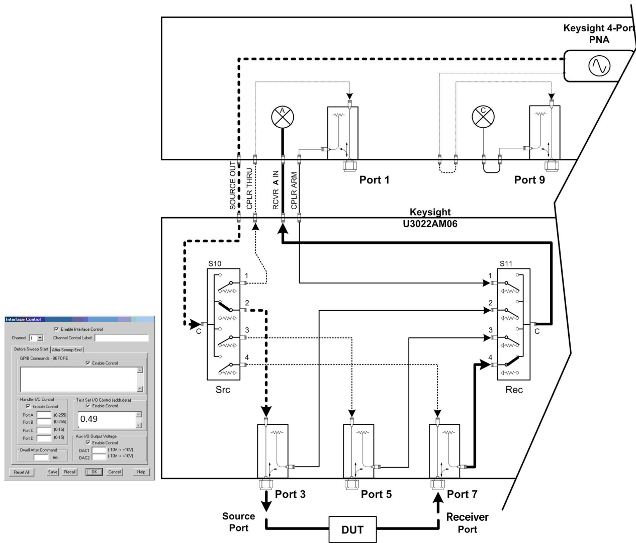
Figure 53 Example - Address and Data (Port 3 and 7)
