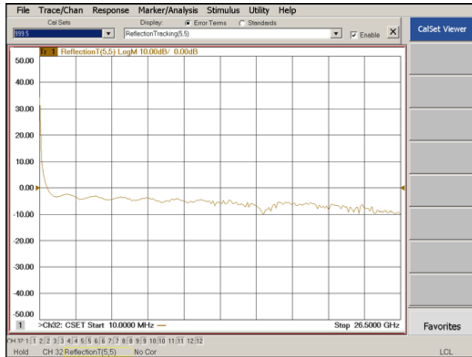
Figure 63 Typical Reflection Tracking Trace with N5242A/B (Ports 3 to 8)
