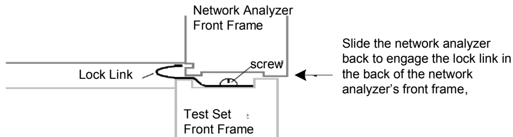
Figure 12 Locking the Analyzer
