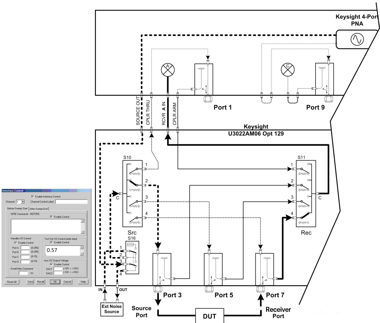
Figure 54 Example 3 - Option 129 Test Port Path Selection
