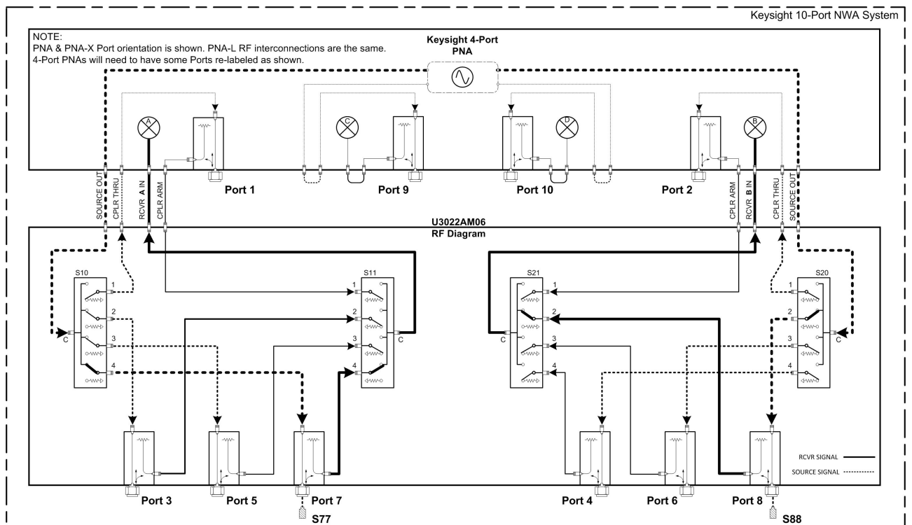
Figure 34 Reflection Response Signal Path Diagram Ports 7- 8
