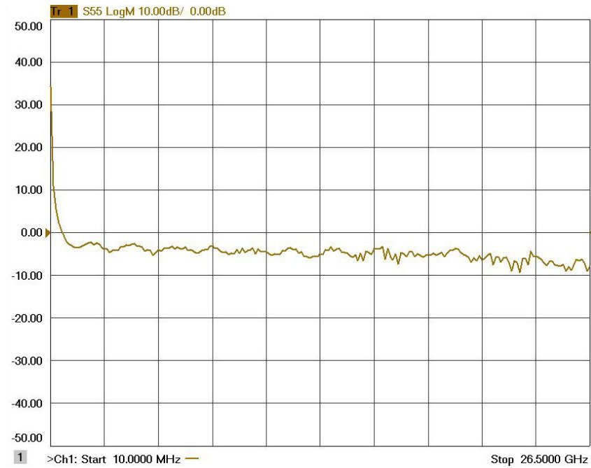
Figure 31 Typical Reflection Response Ports 3-8
