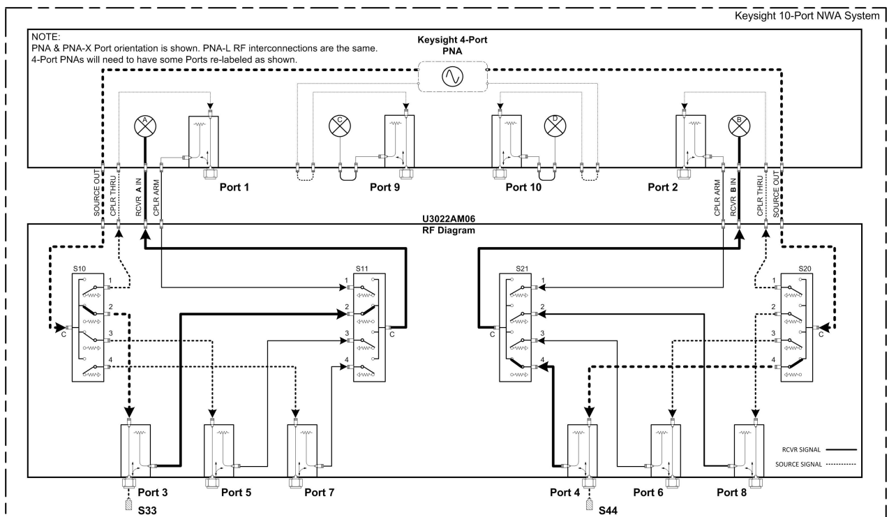
Figure 32 Reflection Response Signal Path Diagram Ports 3-8
