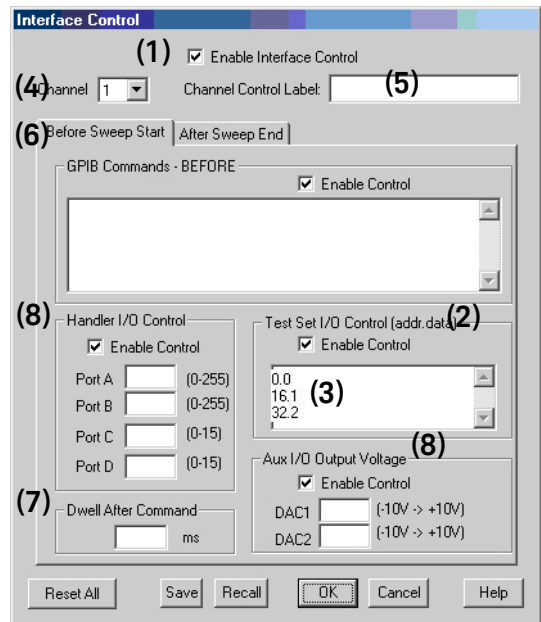
Figure 48 Interface Control
