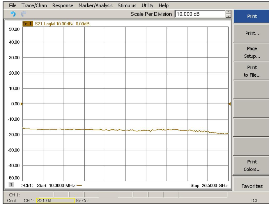
Figure 70 Rcvr Out to Ports 3-8 Path Response
