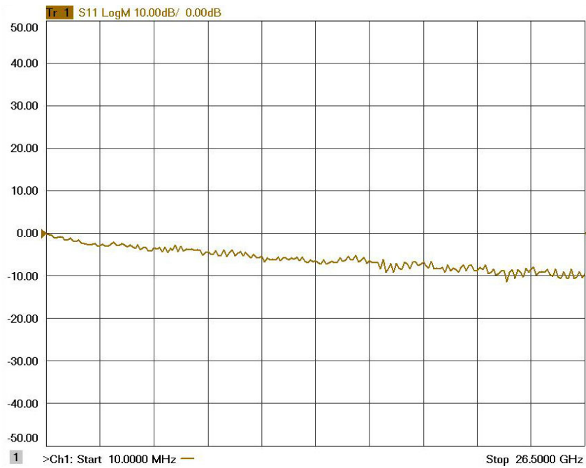
Figure 29 Typical Reflection Response Ports 1-2
