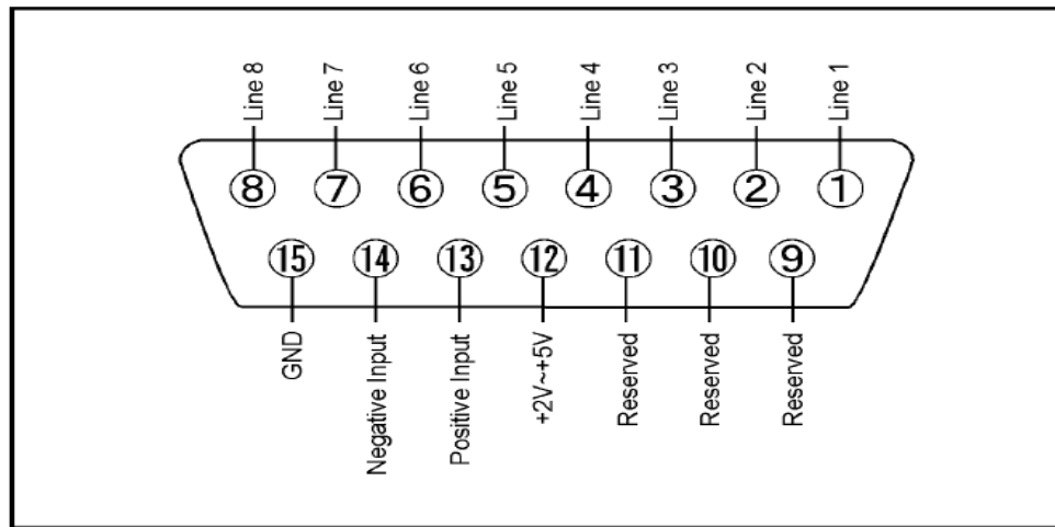
Figure 55 DUT control Line Pin Assignment (rear panel view)
