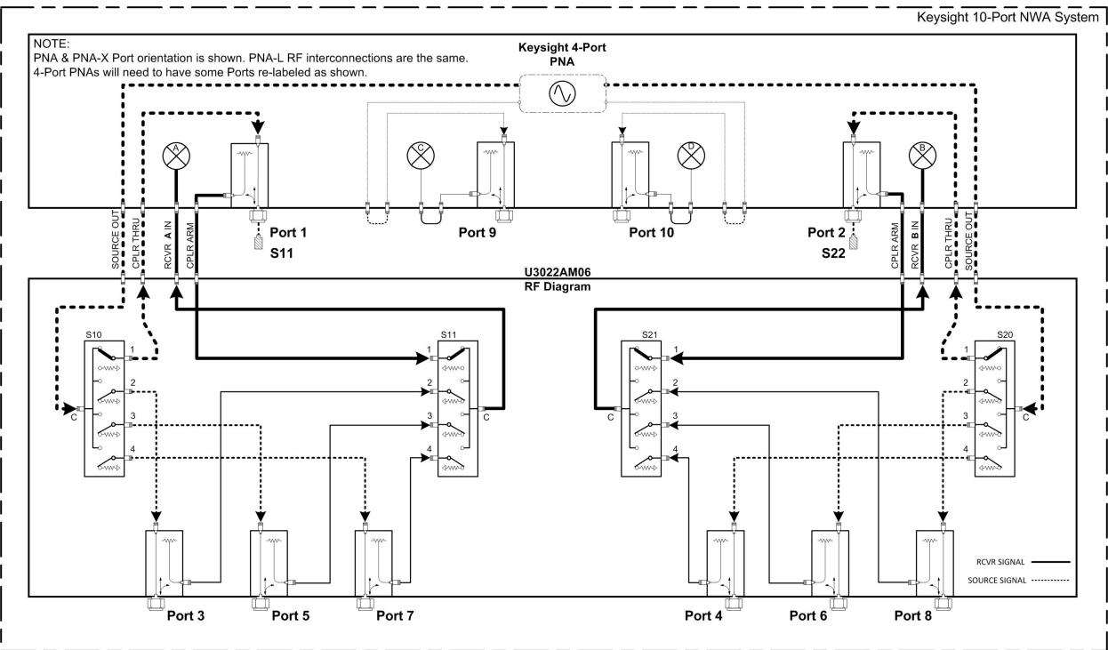
Figure 30 Reflection Response Signal Path Diagram Ports 1-2
