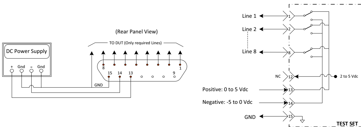
Figure 57 Test Set to the DUT and External DC Power Supply
