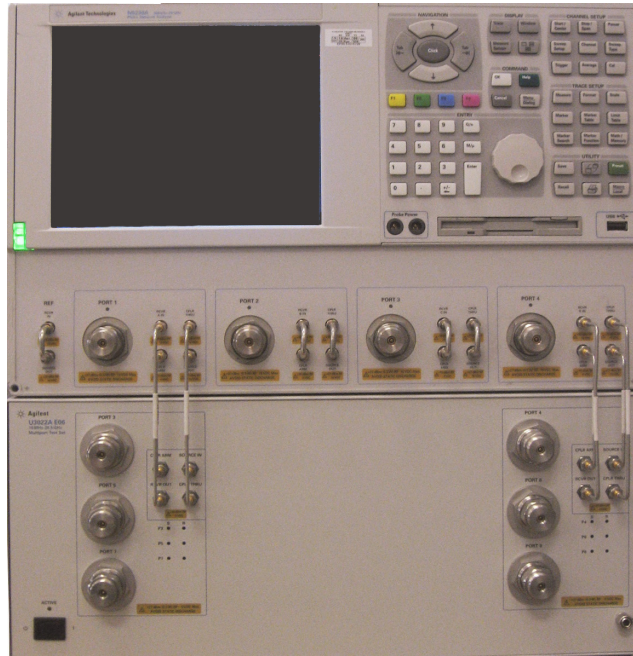
Figure 2 N5230A 4-Port PNA-L with U3022AM06
