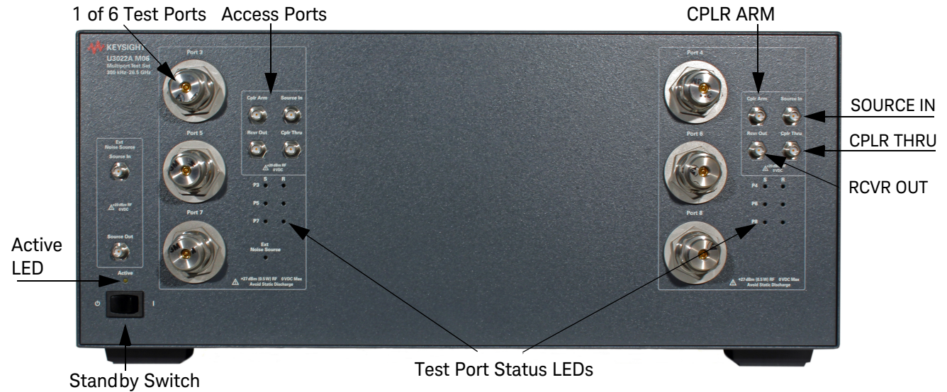
Figure 6 U3022AM06 Front Panel
