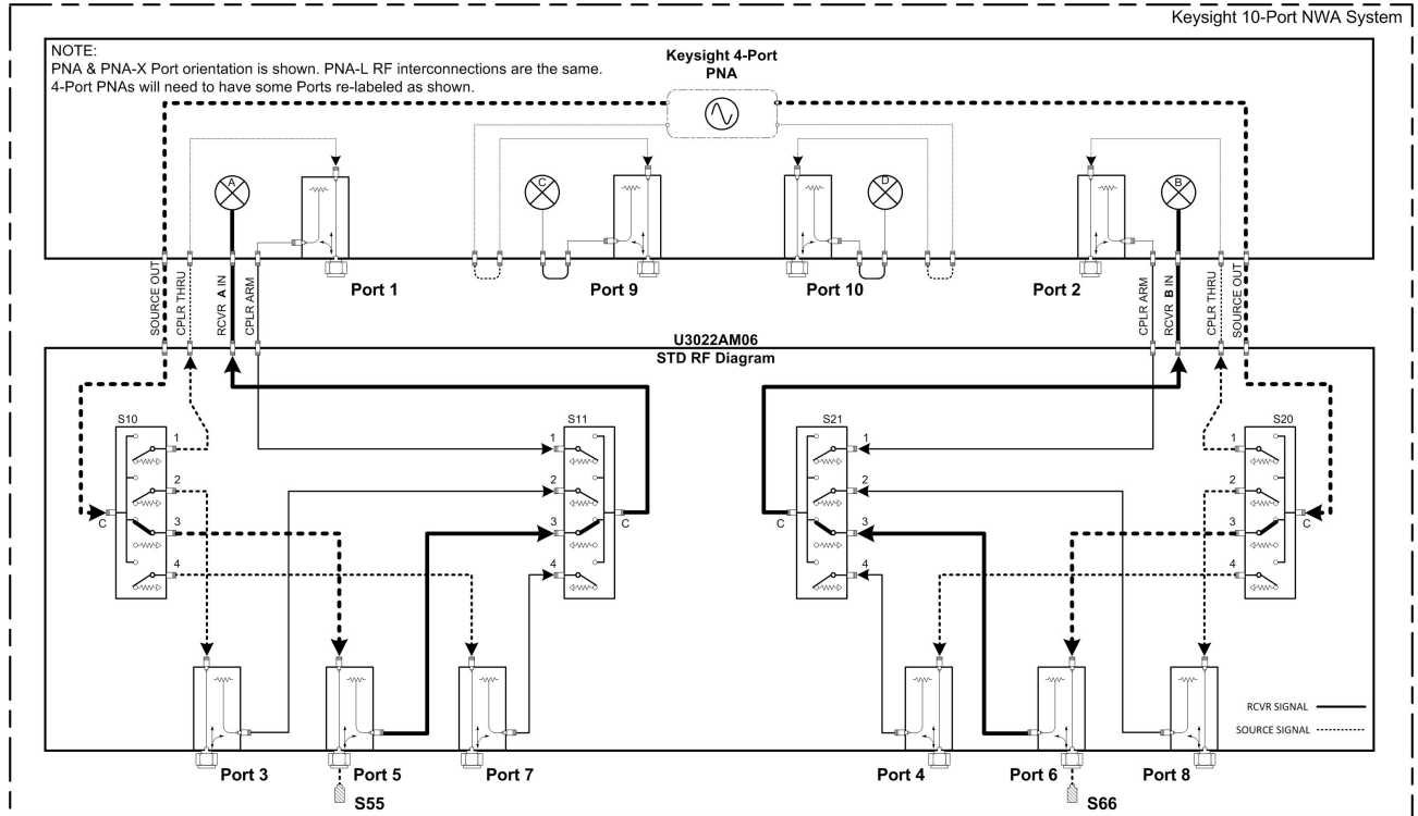
Figure 33 Reflection Response Signal Path Diagram Ports 5-6
