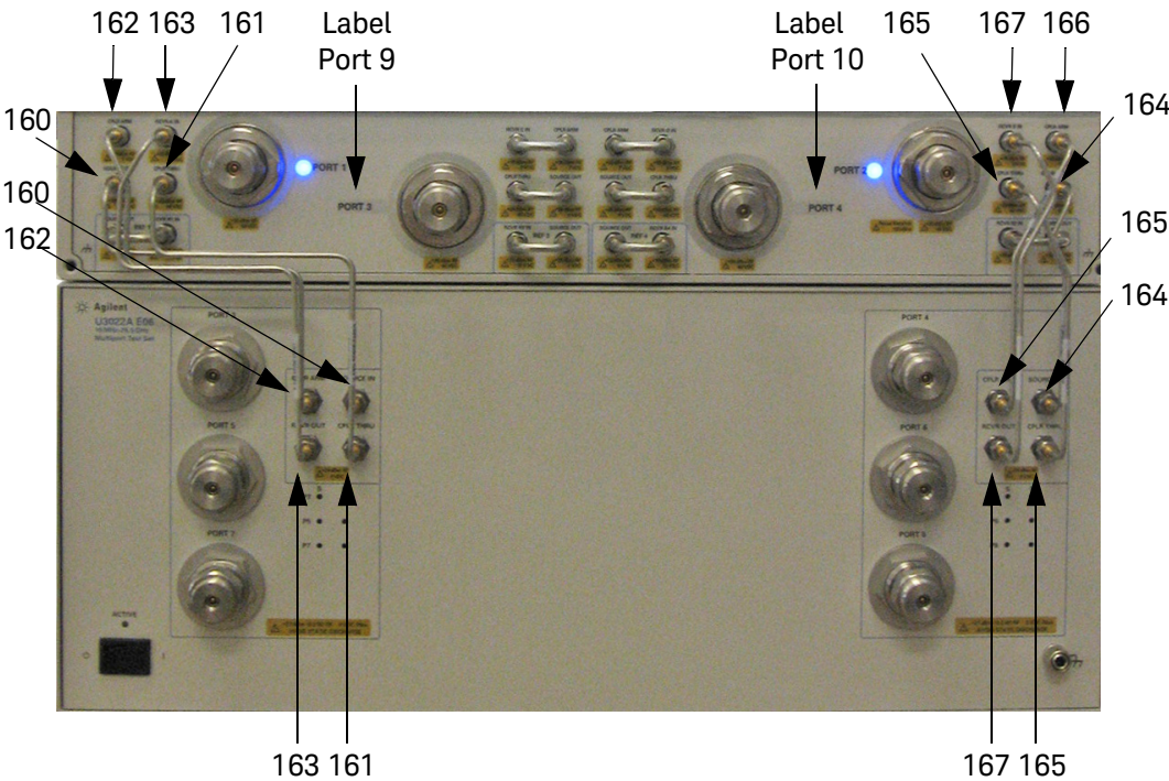
Figure 27 N5247A/B RF Interface Cable Connections
