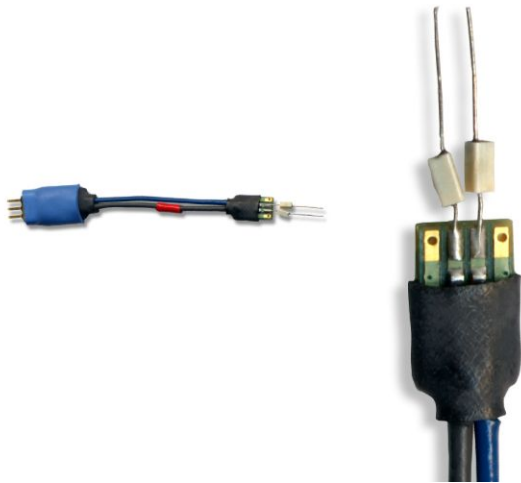
TriMode Micro-coax Tip Low-cost, quick-connect solder tips. Up to 4 GHz bandwidth.
