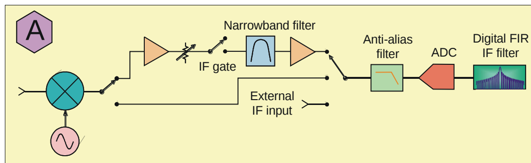
Figure 11. Receiver Block Diagram
