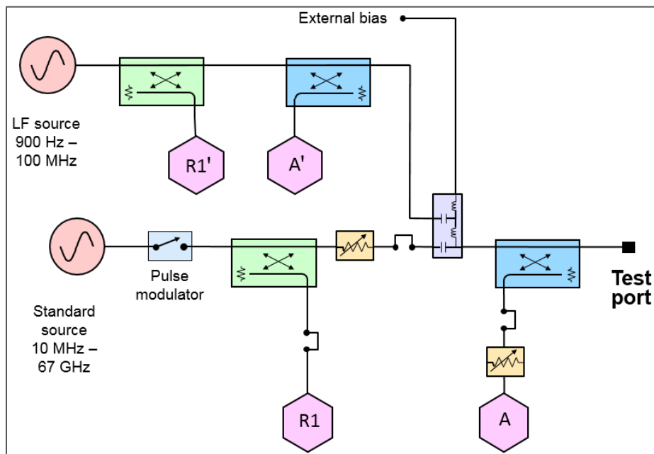
Figure 11. Receiver Block Diagram
