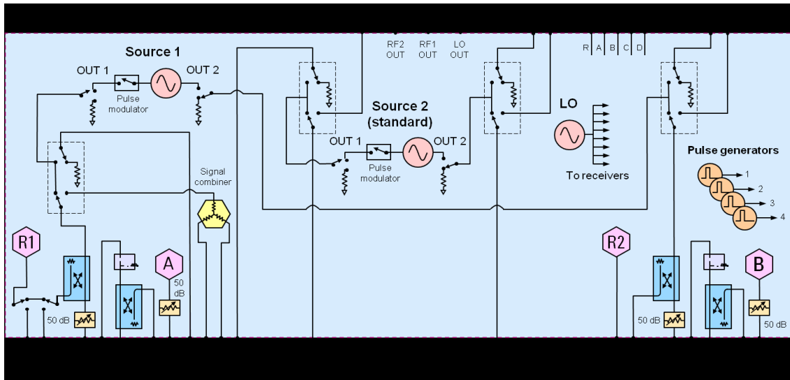
Figure 9. Block Diagram: N5247A Option 224
