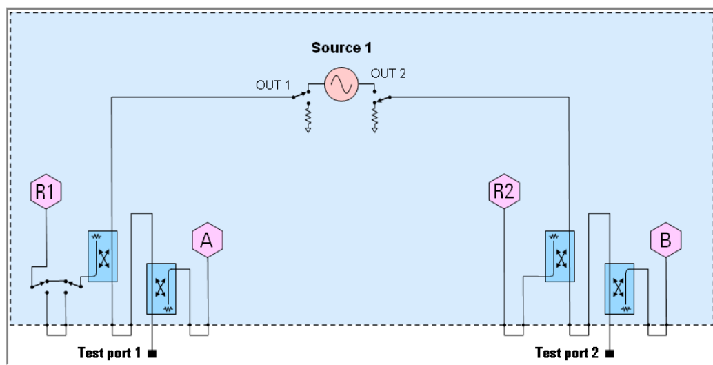
Figure 1. Block Diagram, N5247A Option 200
