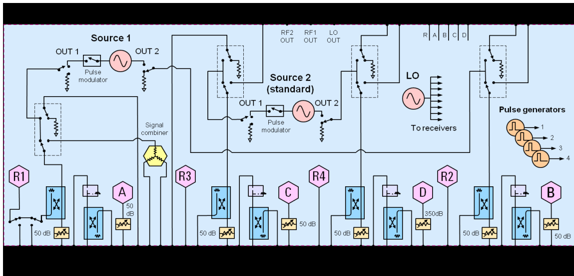
Figure 11. Block Diagram: N5247A Option 423
