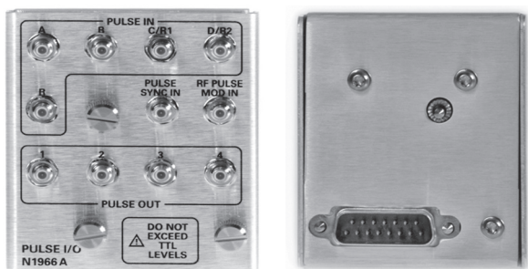
Pulse I/O adapter (N1966A) simplifies connections
