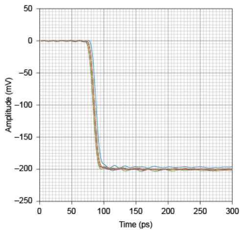
Figure 1. Options 52F, 52M, 54F, and 54M with TDR Calibration (Characteristic)
