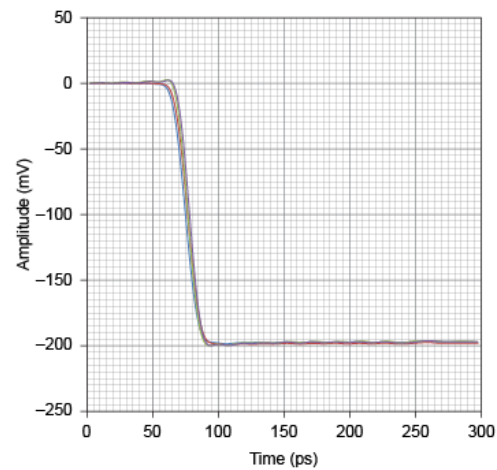
Figure 2. Options 32F, 32M, 34F, and 34M with TDR Calibration (Characteristic)
