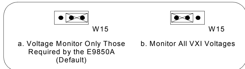
Figure 5-9. Voltage Monitor Settings
