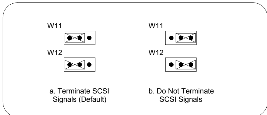
Figure 5-5. SCSI Termination
