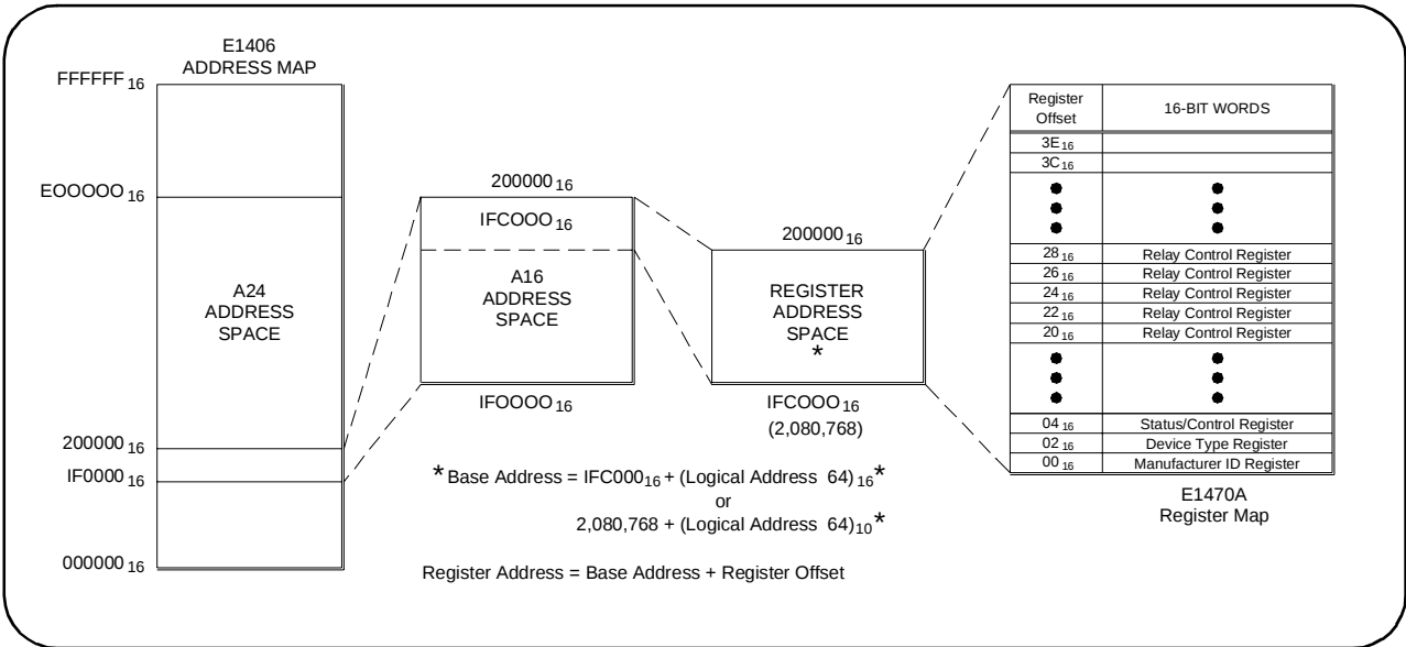
Figure B-2. A16 Address Space in the E1406 Command Module
