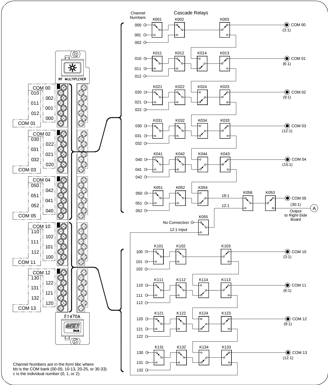
Figure 1-2. Cascade RF Switch Switching Diagram (continued on next page)
