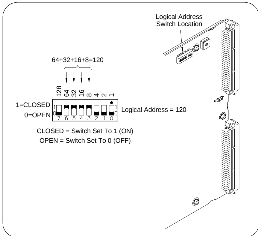
Figure 1-4. Setting the Logical Address Switch
