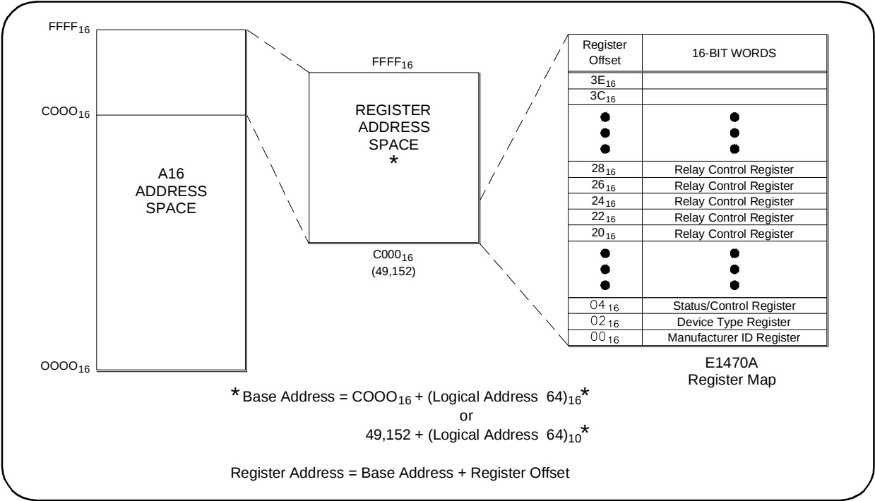
Figure B-1. Register Address Locations Within VXI A16
