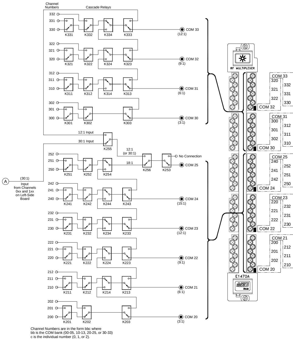
Figure 1-2. Cascade RF Switch Switching Diagram (continued)
