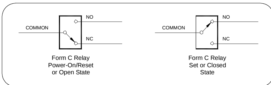
Figure 1-1. Form C Relays States
