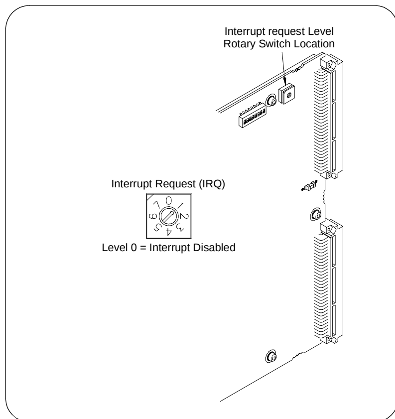
Figure 1-5. Setting the Interrupt Request Level Switch
