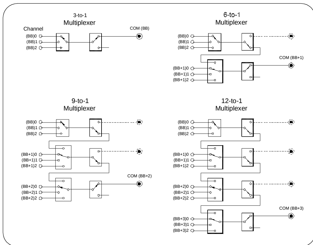
Figure 1-3. Creating Multiple Multiplexers
