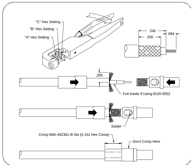
Figure 1-7. Assembling SMB Jacks and Cables
