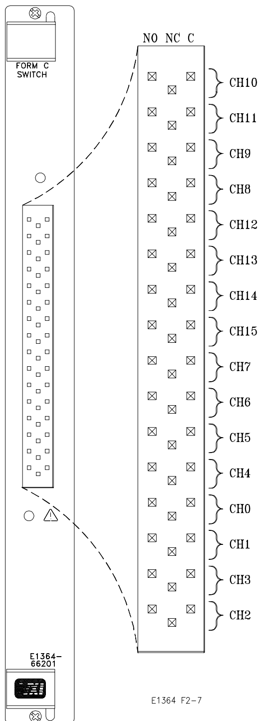
Figure 2-7. E1364A Front Panel and Wiring Diagram
