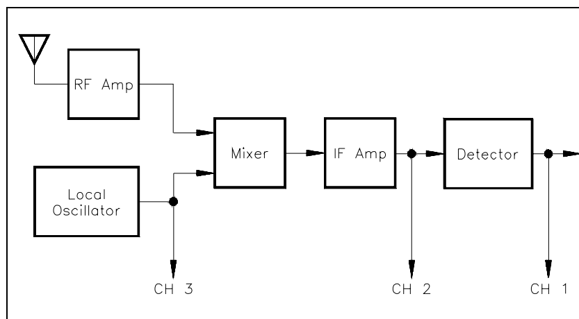
Figure 3-4. Frequency Measurement
