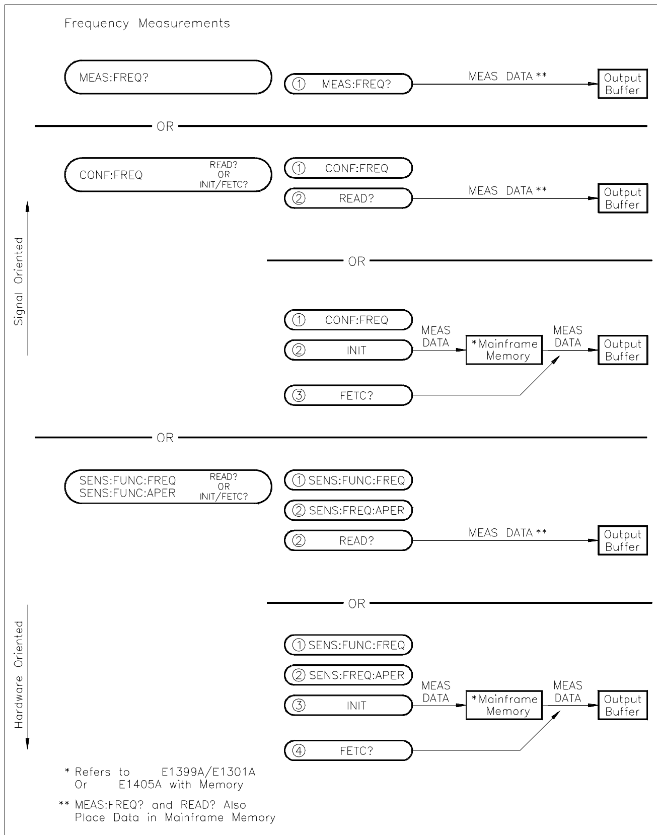
Figure 4-1. Measurement Commands
