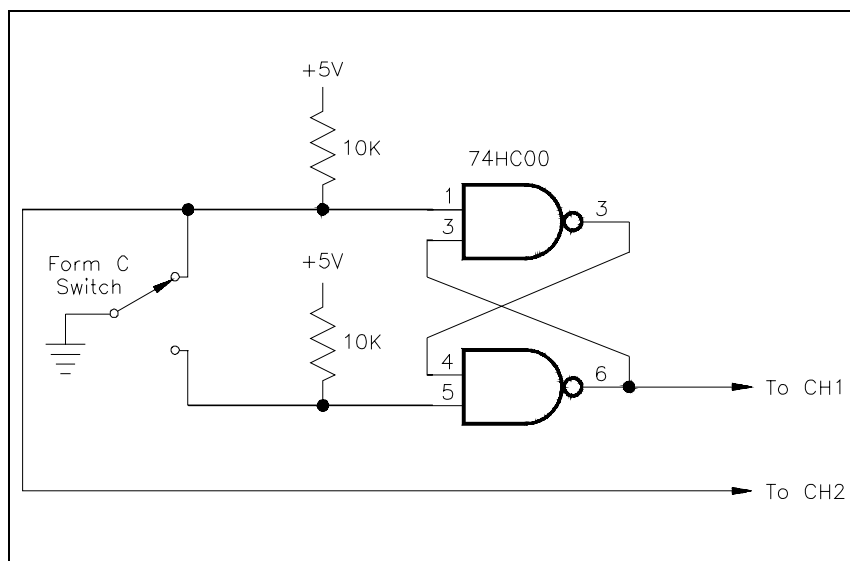
Figure 3-3. Counting Events (Totalize)
