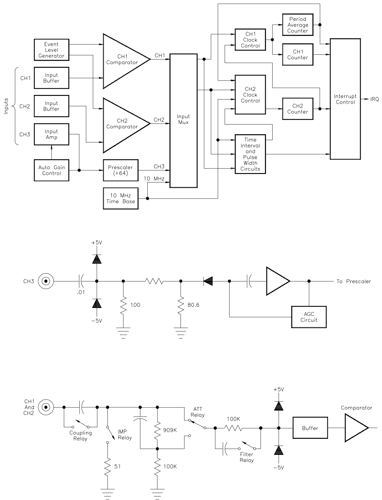
Figure 1-1. Universal Counter Block Diagram
