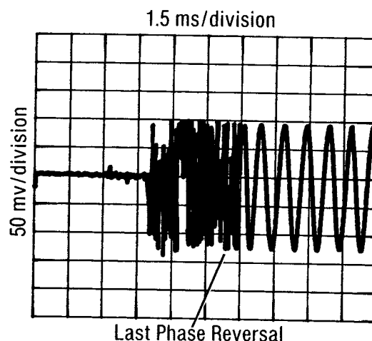
Figure 4-3. Frequency Switching Time Measurement Waveform
