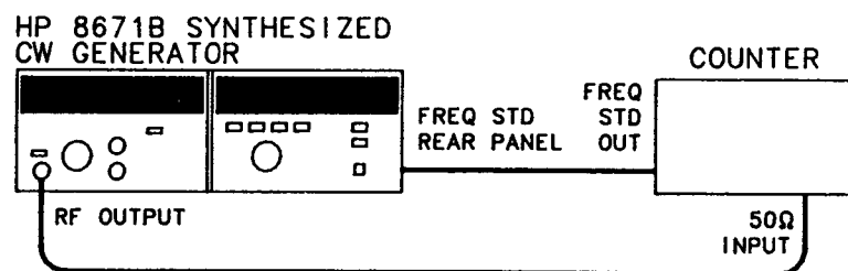
Figure 4-1. Frequency Range and Resolution Test Setup
