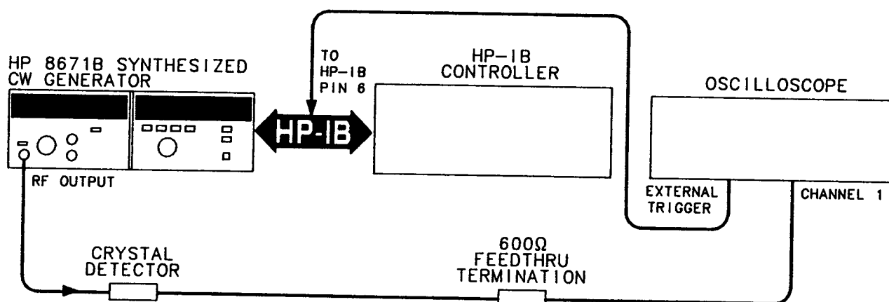
Figure 4-7. Output Level Switching Time Test Setup
