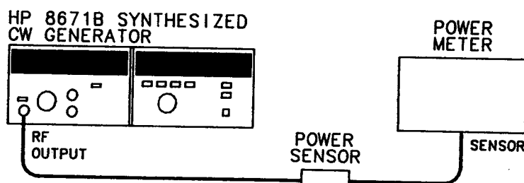
Figure 4-5. Output Level, High Level Accuracy and Flatness Test Setup
