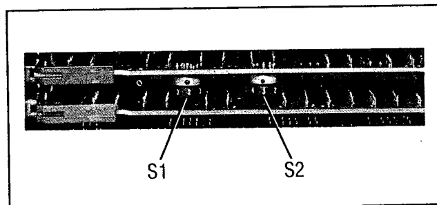
Figure 2-3. HP-IB Address Switches Shown as Set by the Factory
