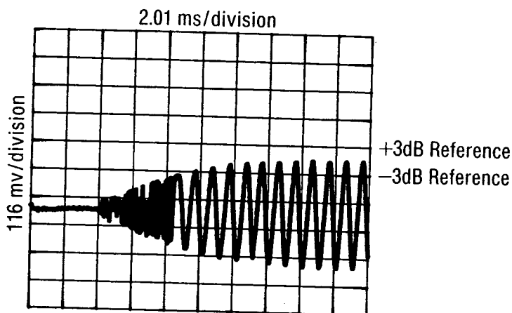
Figure 4-4. Amplitude Recovery Measurement Waveform
