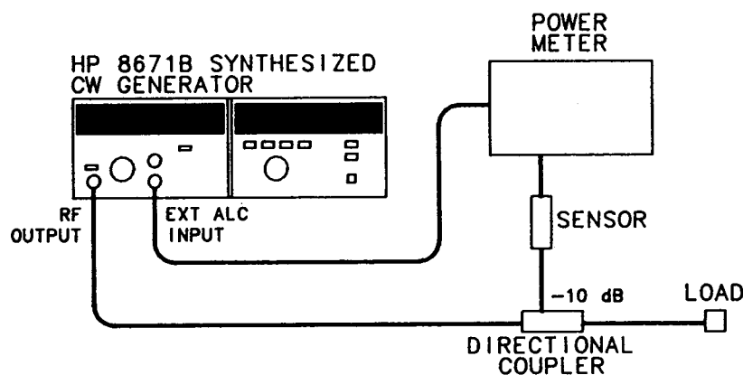
Figure 3-4. External Leveling with a Power Meter
