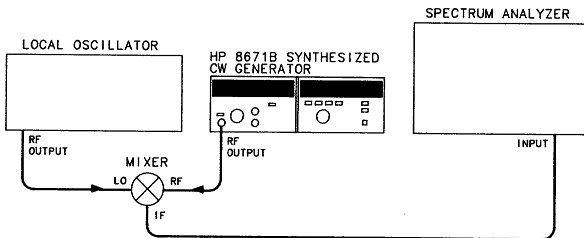
Figure 4-12. Single-Sideband Phase Noise Test Setup
