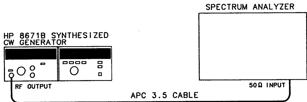
Figure 4-9. Harmonics, Subharmonics, and Multiples Test Setup
