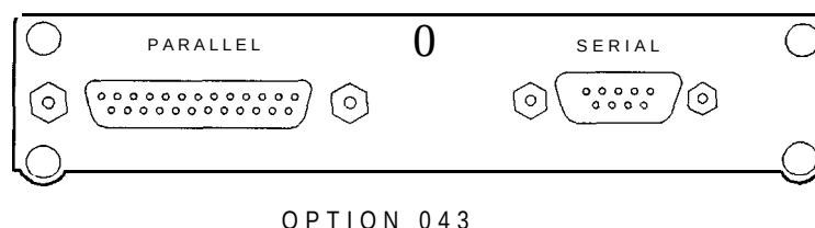
Figure C-1. RS-232 Connector
