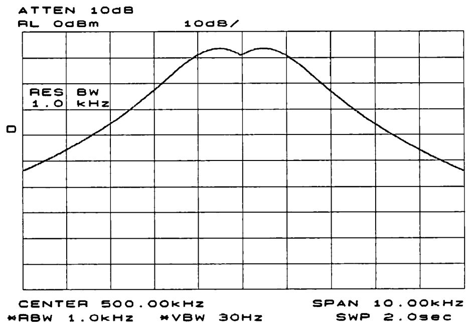
Figure 3-15. 1 kHz Signal Separation
