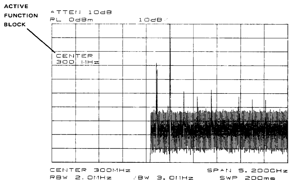
Figure 1-5. Center Frequency Set to 300 MHz
