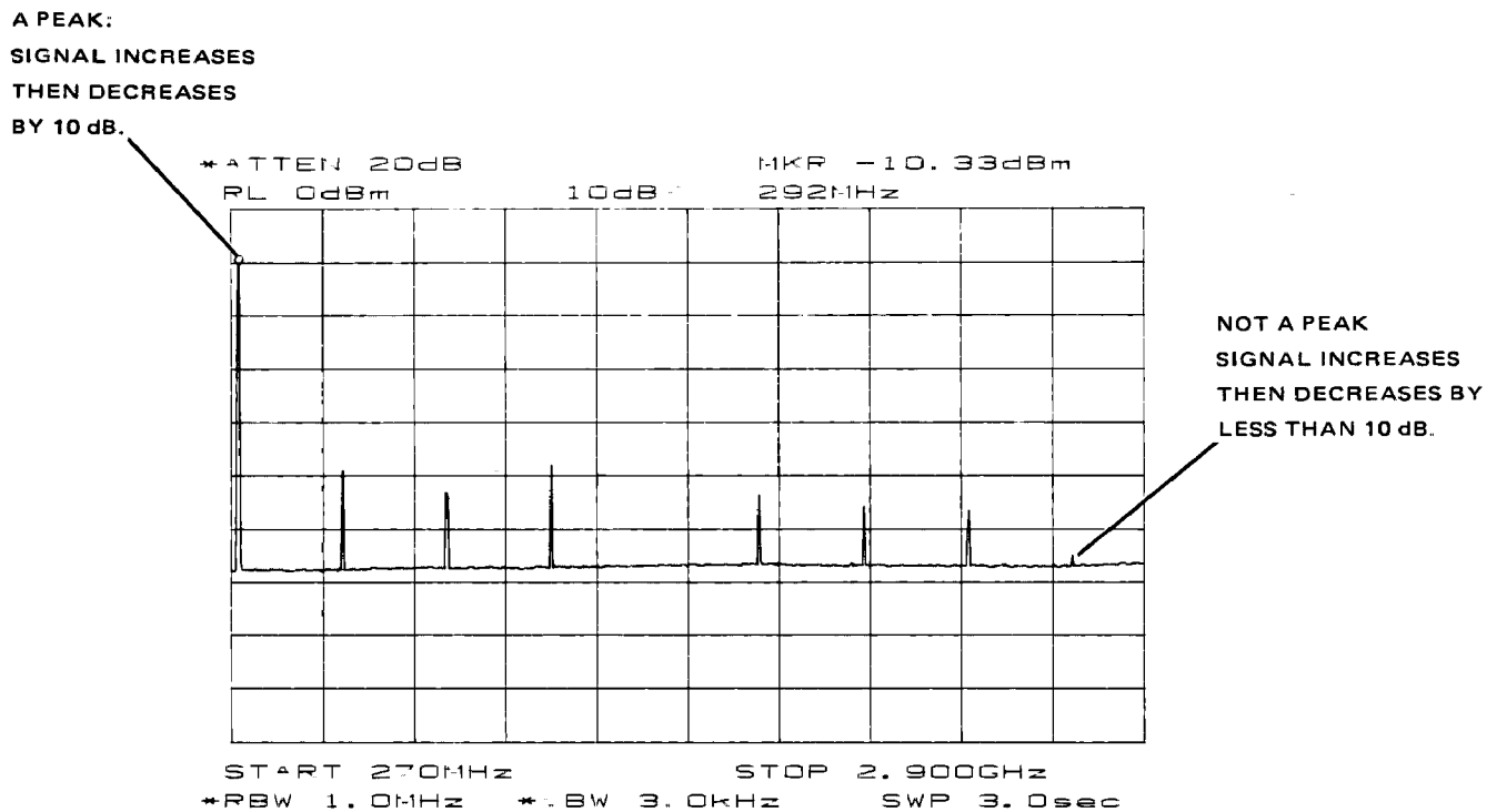
Figure 5-3. MKPX Determines Which Signals are Considered Peaks
