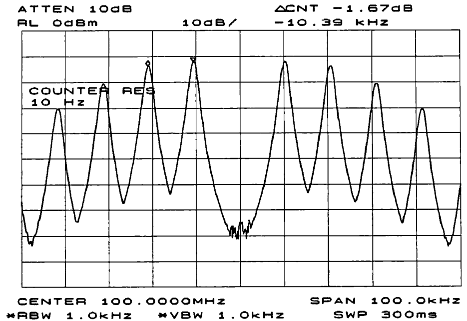
Figure 3-27. Markers Show Modulating Frequency
