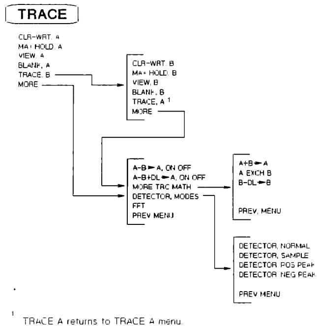
Figure 2-23. TRACE Menu
