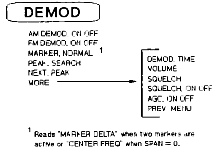
Figure 2-13. DEMODO Menu
