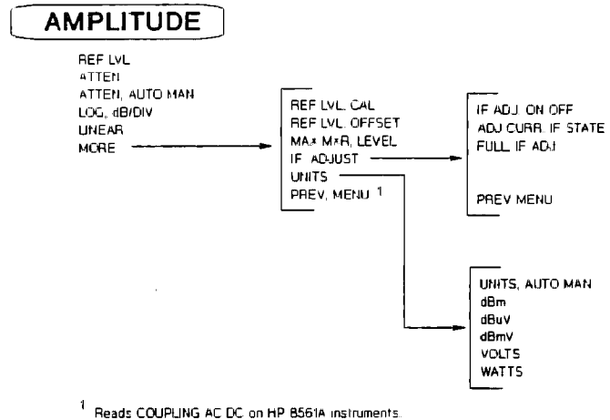
Figure 2-4. AMPLITUDE Menu
