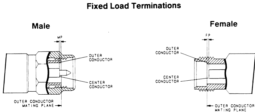
Figure 2-1. 3.5 mm Center Conductor Recession
