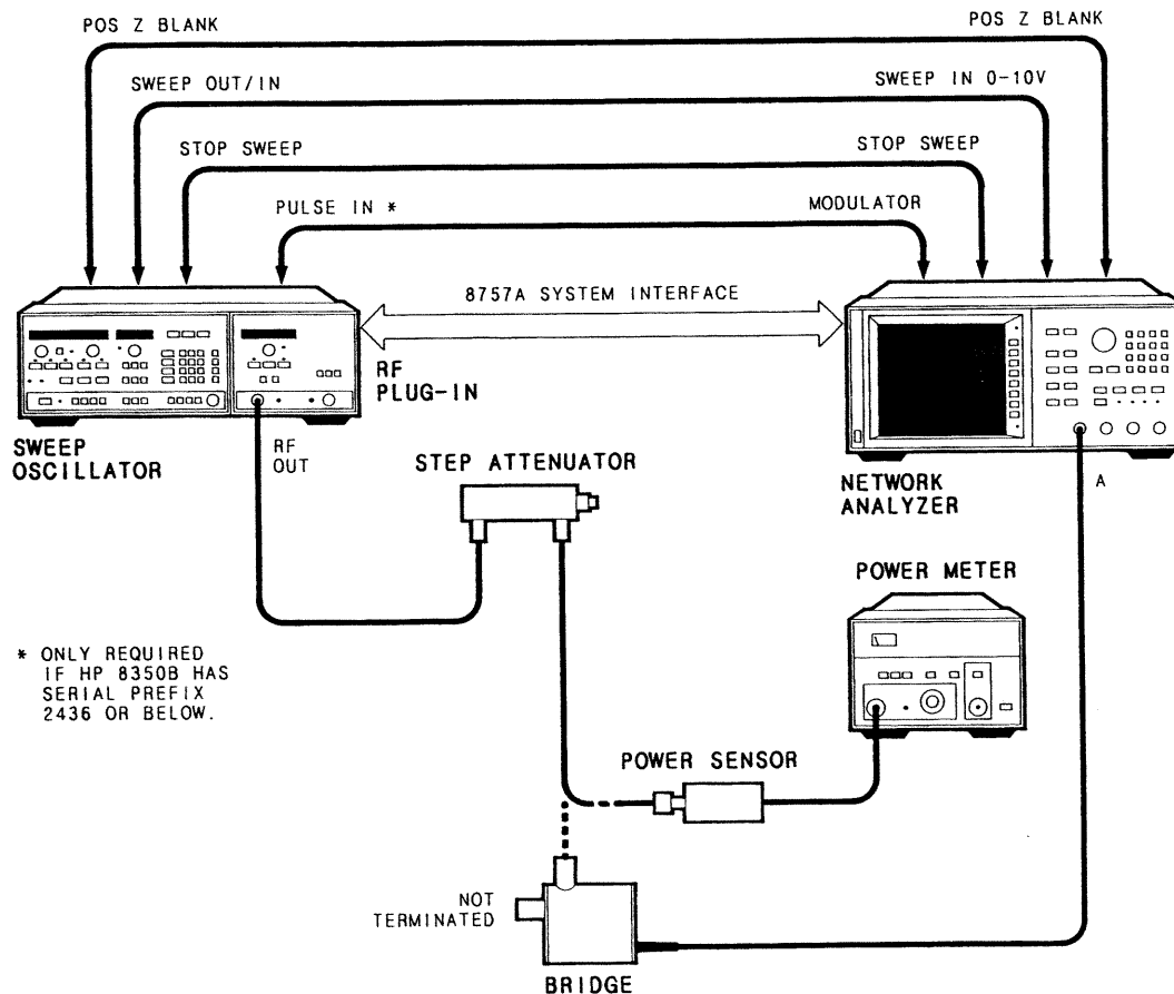
Figure 5-1. Adjustment Setup
