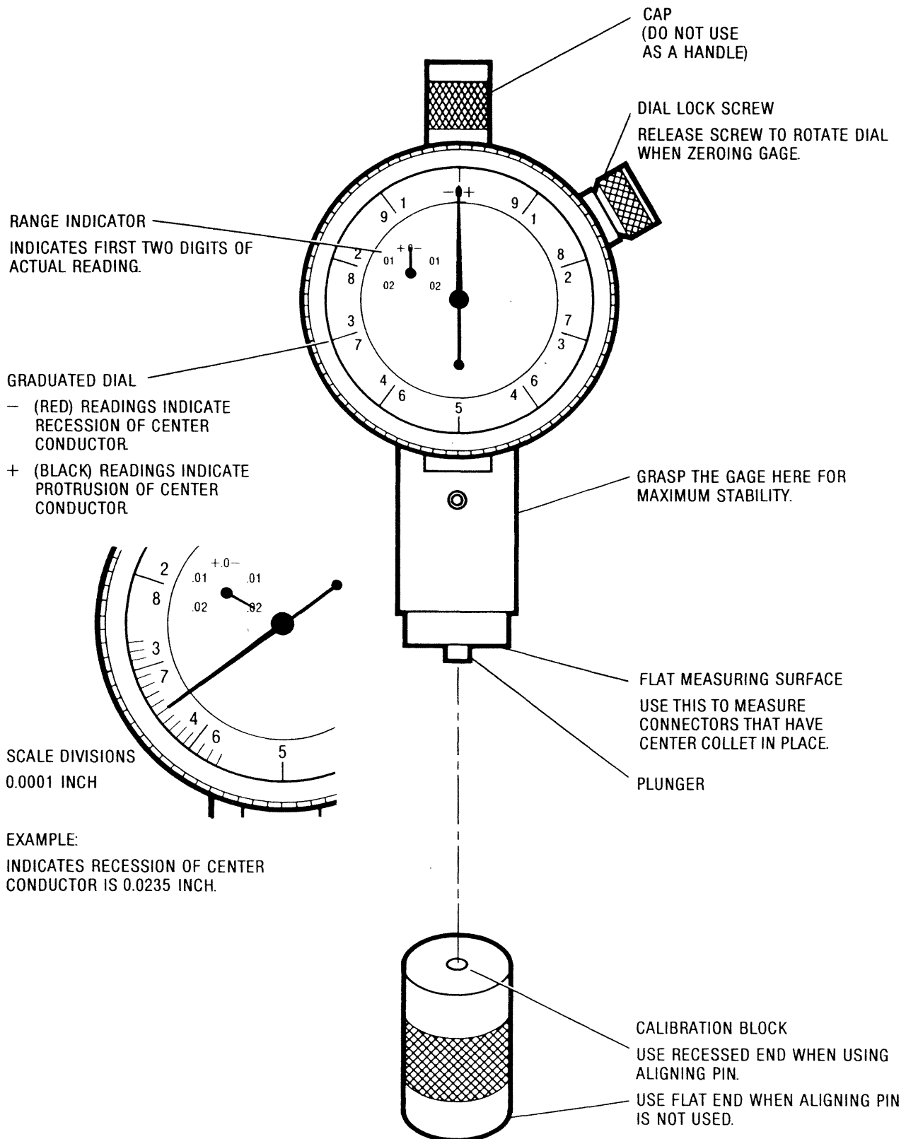
Figure 8-8. The APC-7 Connector Gage
