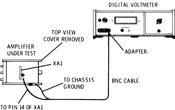
Figure 10. Power Supply Voltage Adjustment Test Setup
