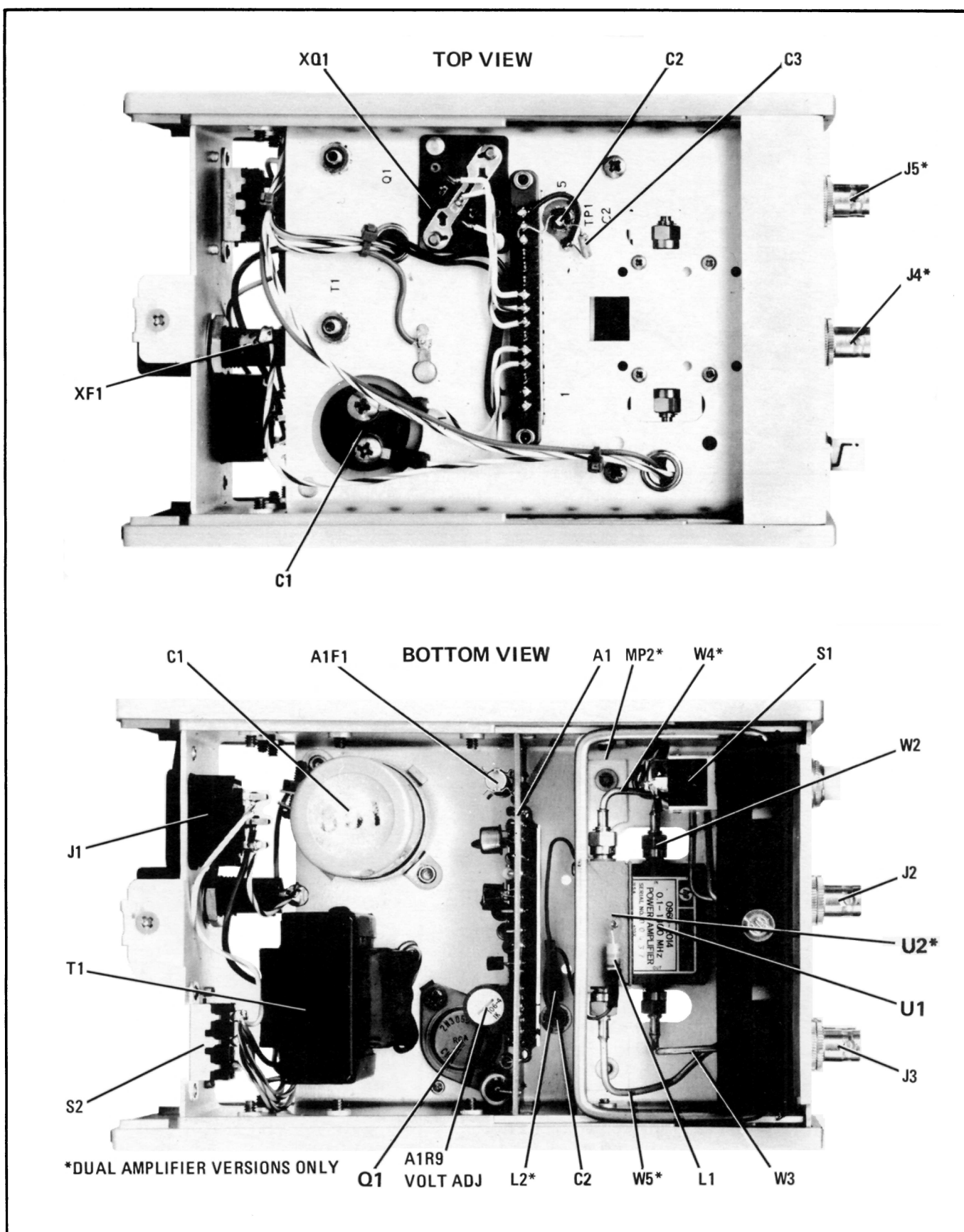
Figure 13. Internal Views
