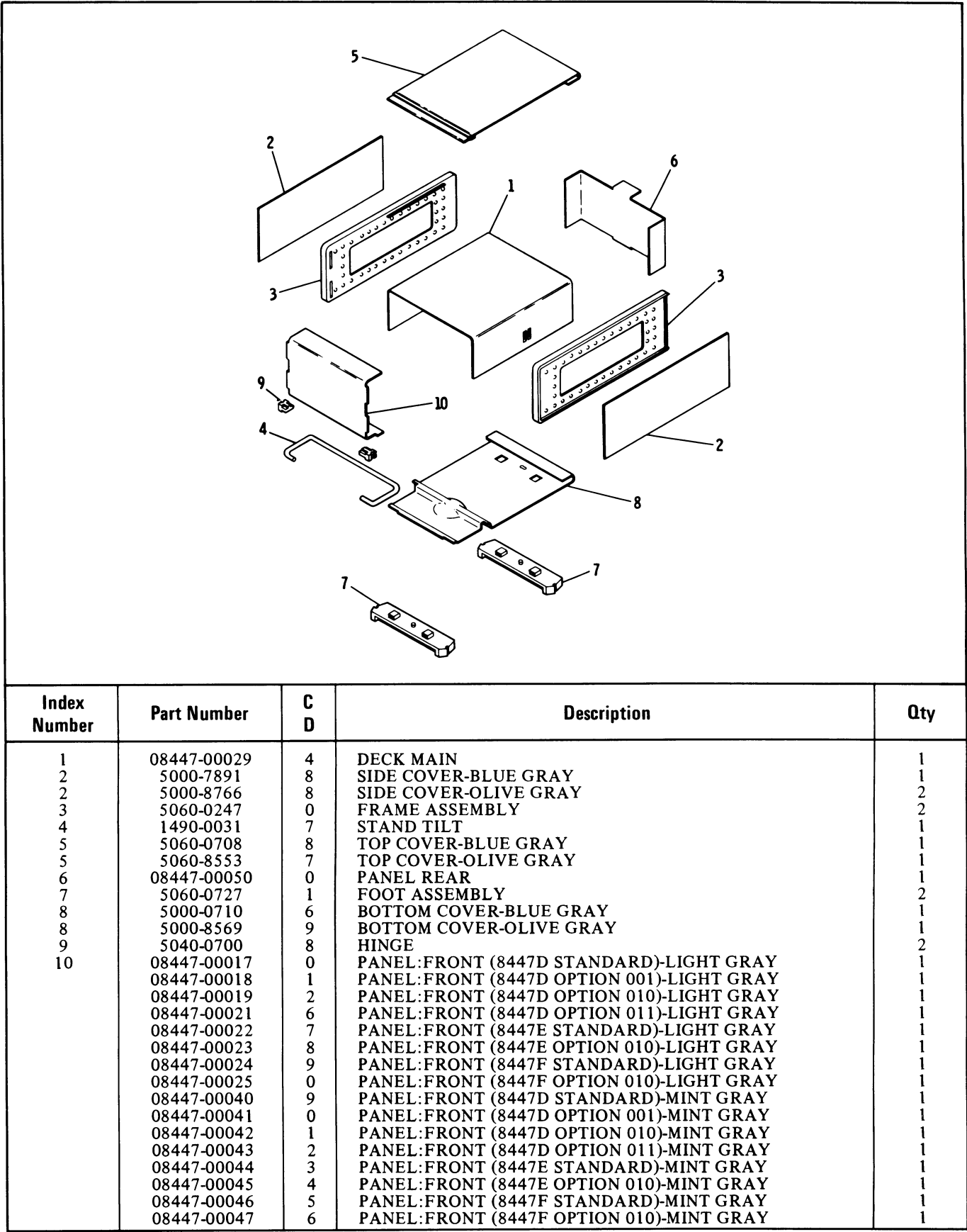
Figure 11. 8447D/E/F Cabinet Parts
