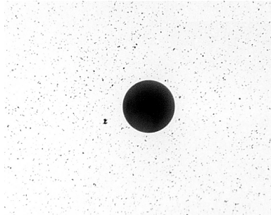
Figure 3-5. Clean, problem-free fiber end and ferrule.
