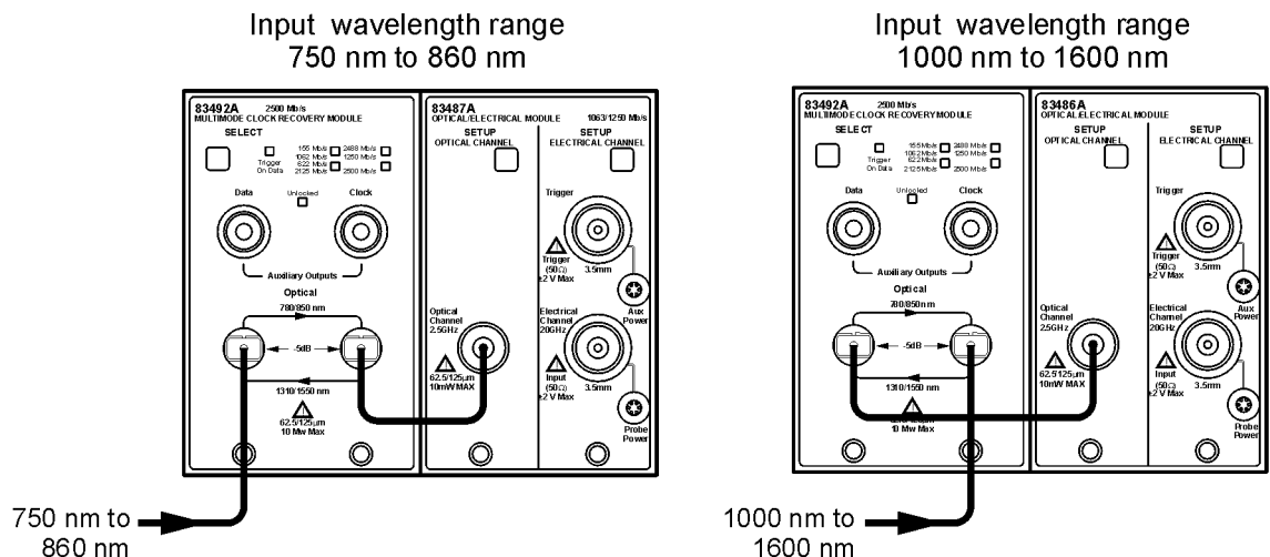
Figure 1-4. Input and output connections versus wavelength
