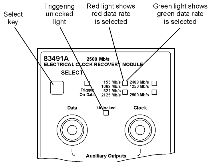
Figure 1-5. Front-panel lights
