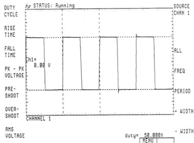
Figure 2-82. DUTY CYCLE Enabled
