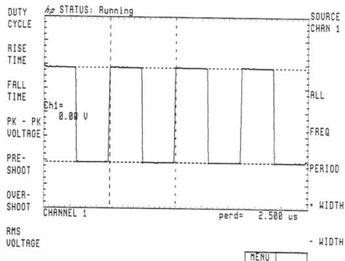
Figure 2-79. PERIOD Enabled
