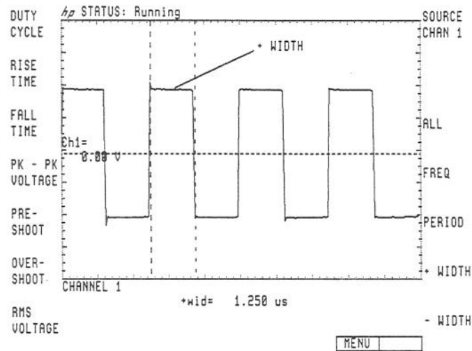
Figure 2-80. + WIDTH Enabled
