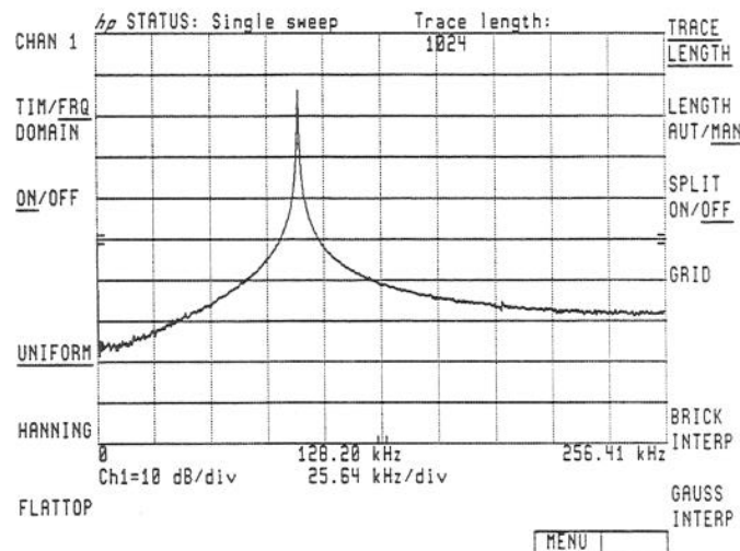
Figure 2-52. UNIFORM Window
