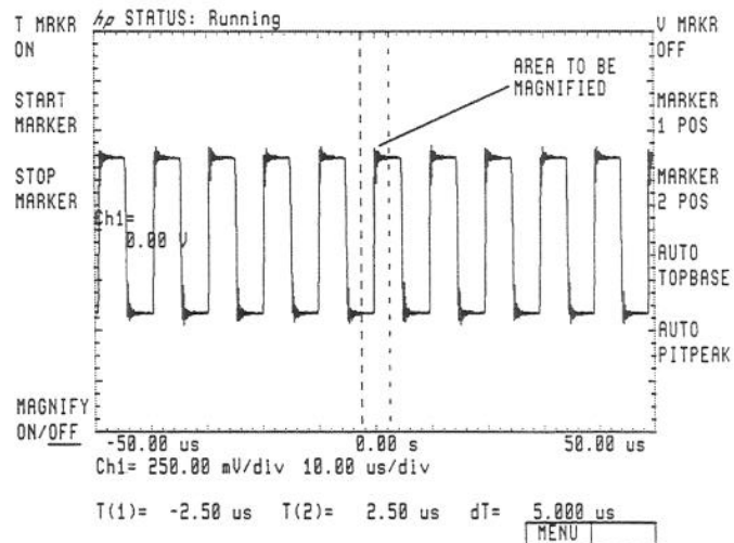
Figure 2-68. START and STOP Markers Positioned for Magnification
