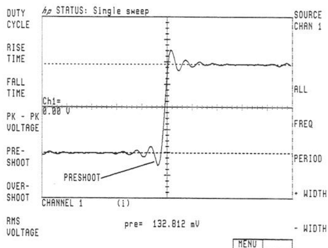
Figure 2-86. PRESHOOT Enabled
