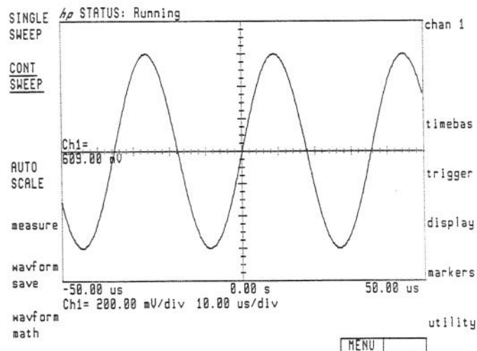
Figure 2-75. Displayed Waveform AUTO-SCALED
