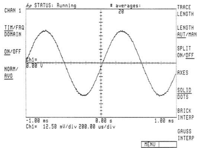
Figure 2-58. AVERAGED Waveform
