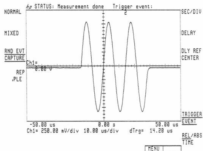
Figure 2-20. Trigger Event #2
