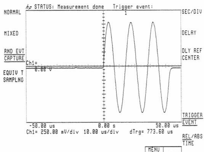
Figure 2-19. Trigger Event #1
