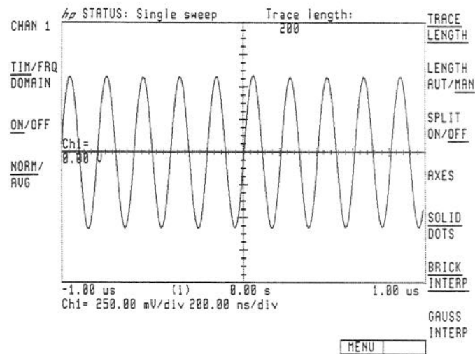
Figure 2-47. Sine Wave with Brick Interpolation
