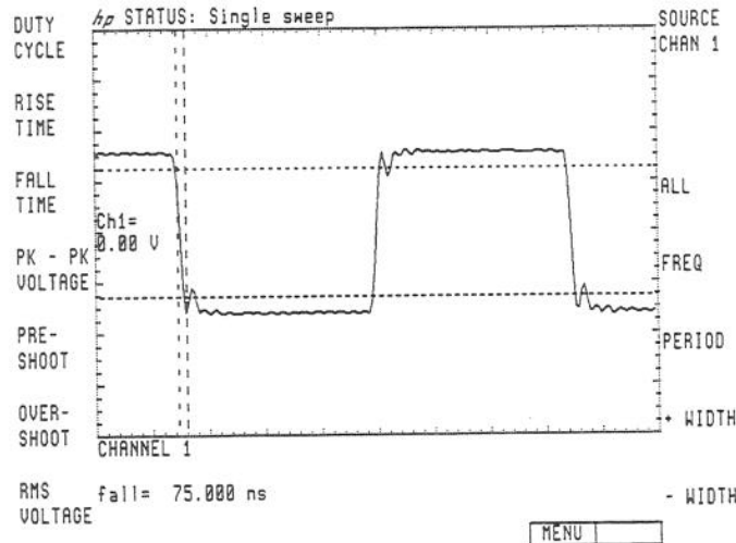
Figure 2-84. FALL TIME Enabled
