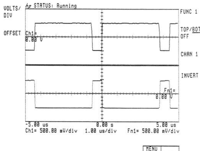
Figure 2-96. CHANNEL 1 INVERTED
