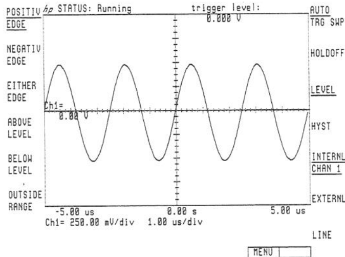
Figure 2-26. TRIGGER Softkeys
