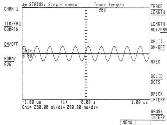
Figure 2-48. Sine Wave with Gaussian Interpolation
