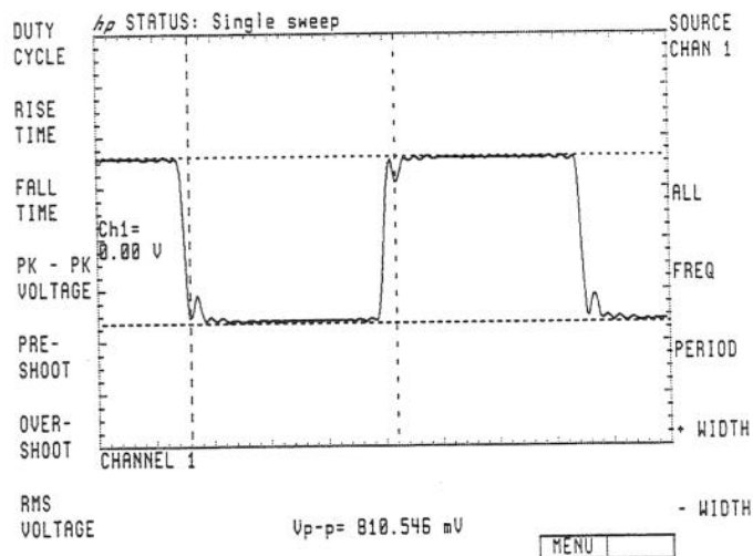
Figure 2-85. PEAK-TO-PEAK VOLTAGE Enabled
