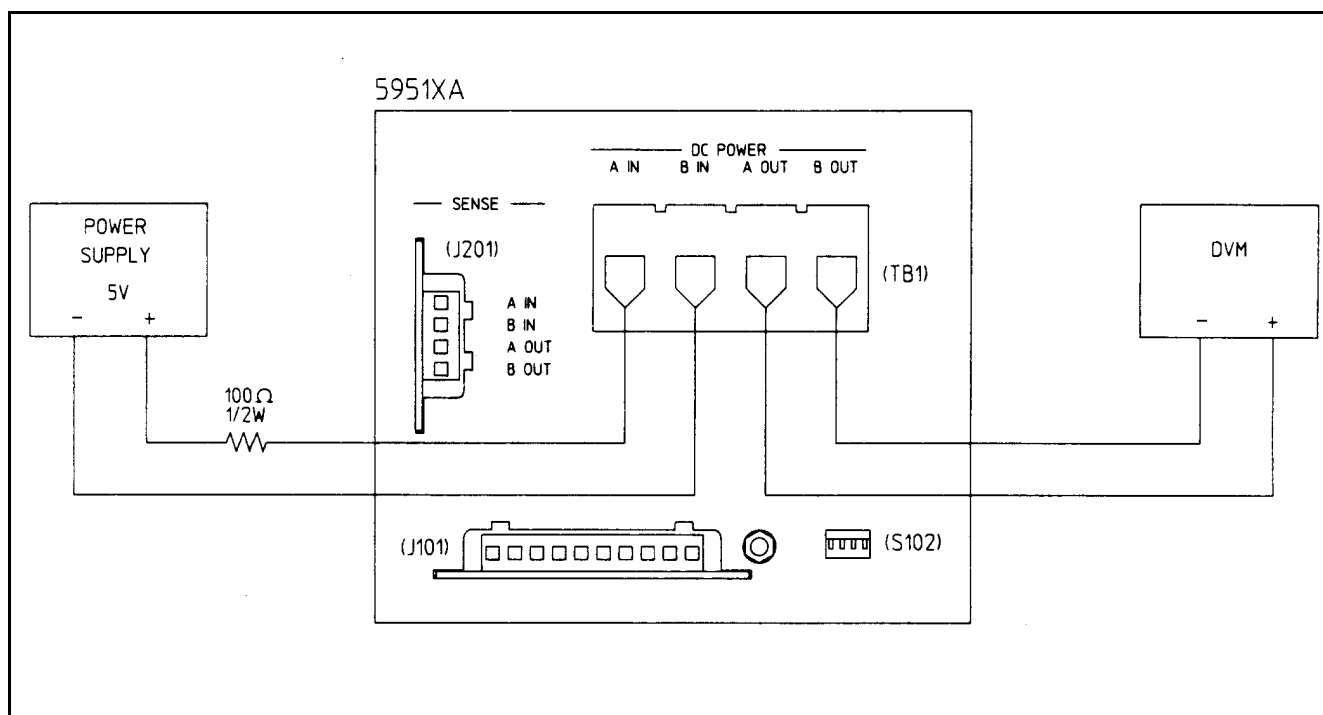
Figure 5-3. DC Power Relay Verification Test Setup
