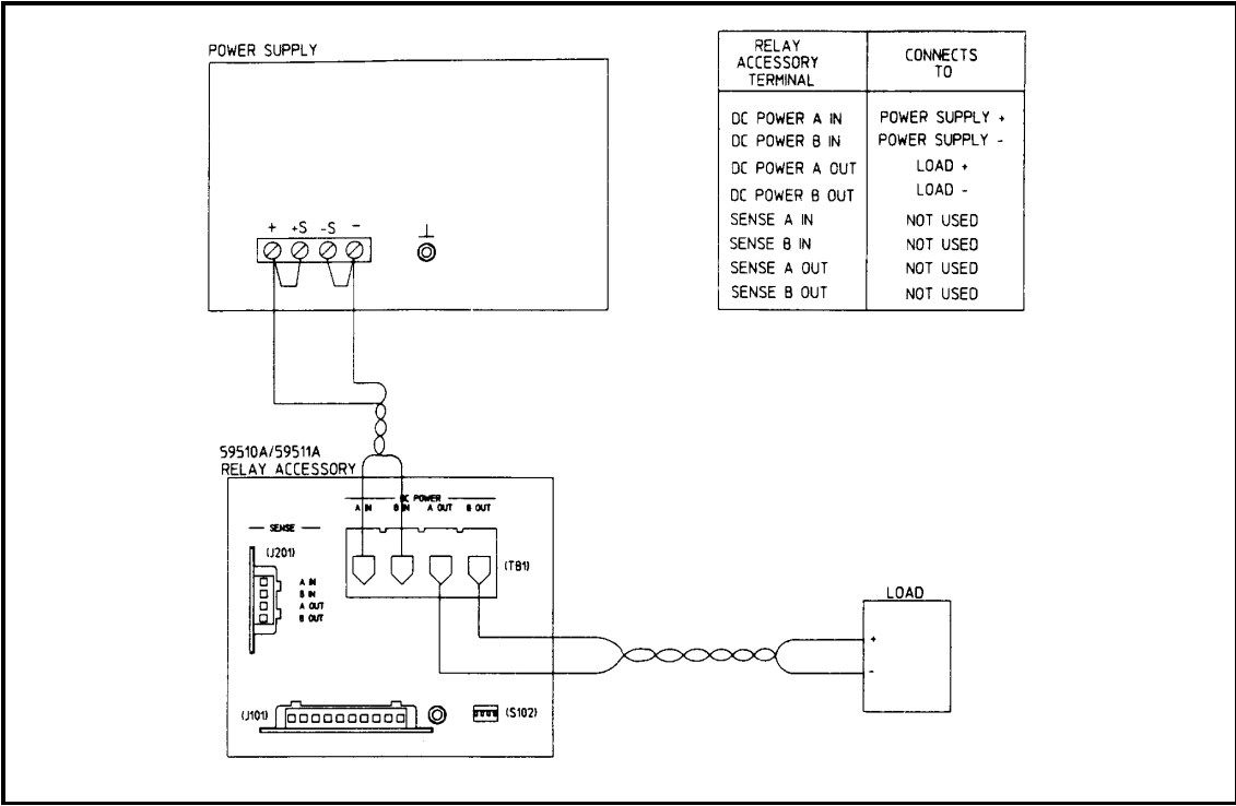
Figure 3-3. DC Power and Sense Lead Connections, Local Sensing
