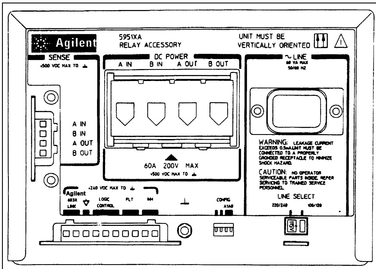
Figure 2-3. Relay Accessory Front Panel
