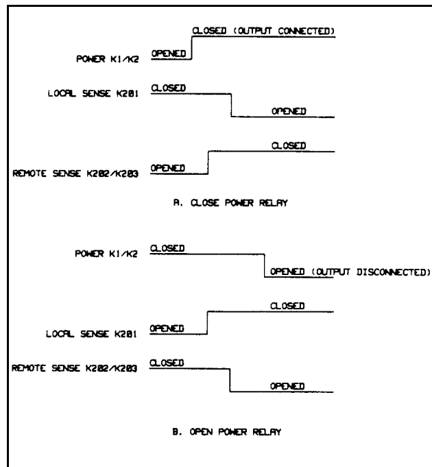
Figure 5-1. Relay Timing
