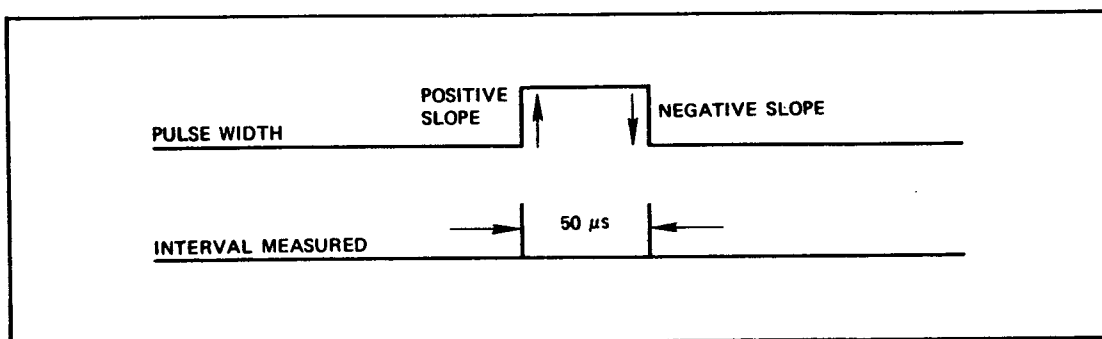
Figure 3-4. SLOPE Switch Settings
