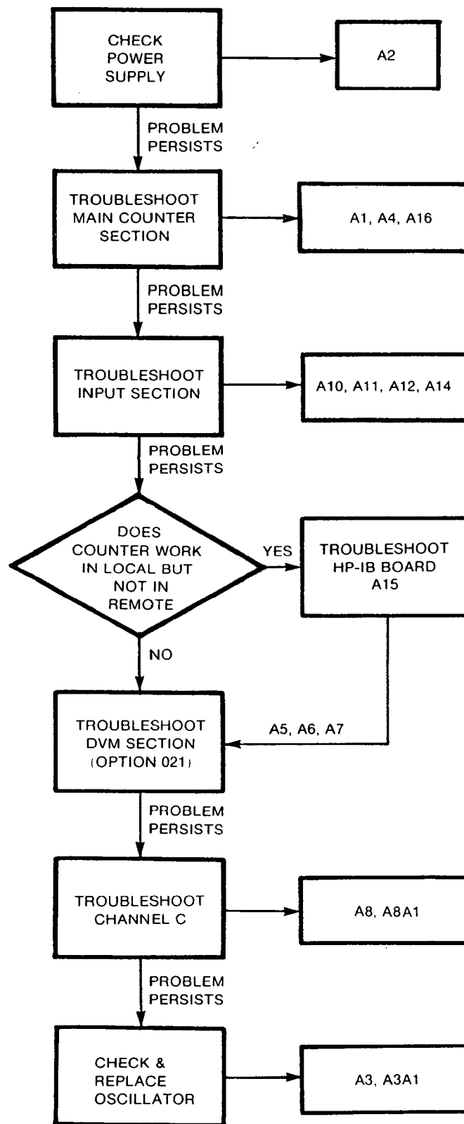
Figure 8-10. Sequential Mode Troubleshooting
