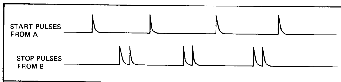
Figure 3-10. Time Interval Measurements — Multiple STOP Pulses
