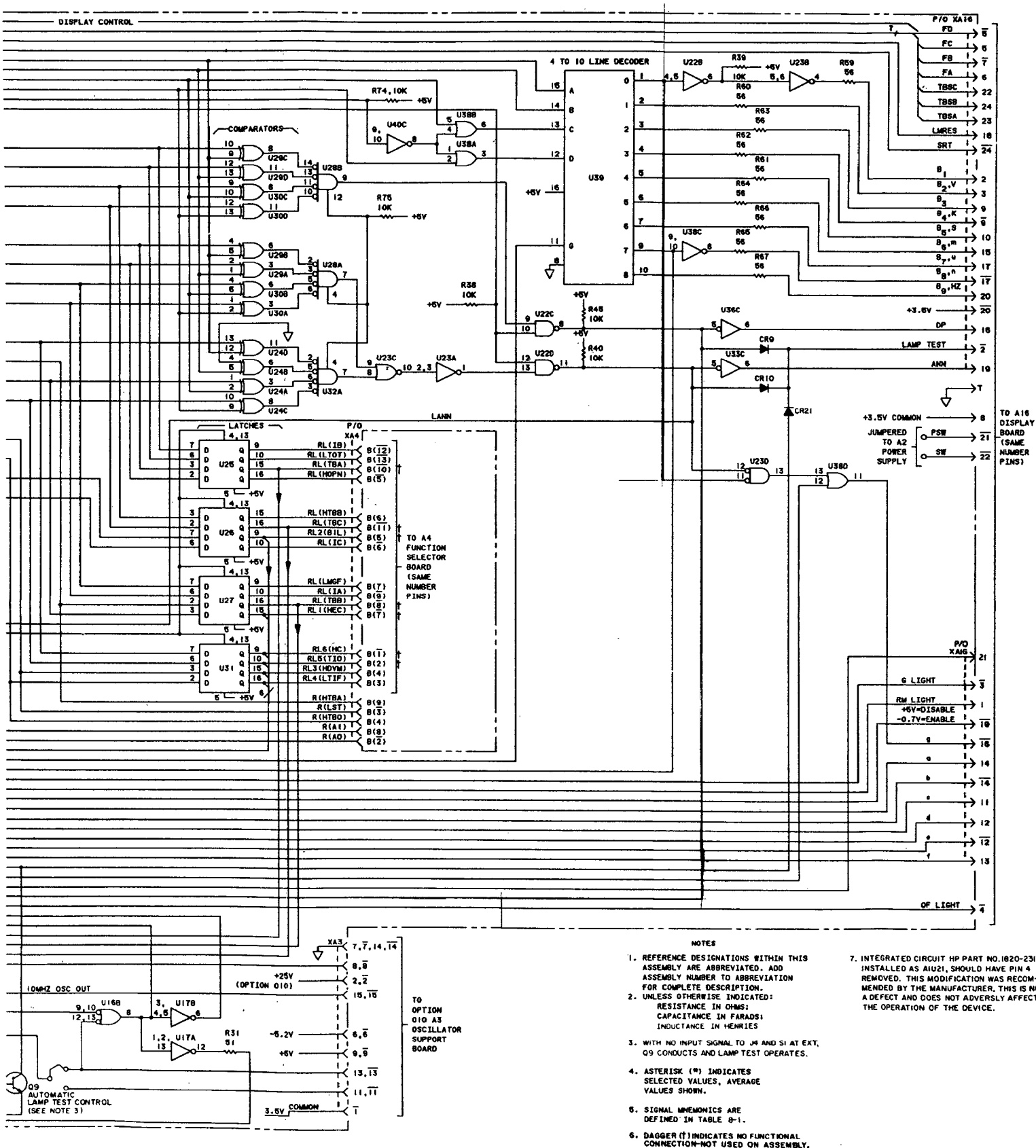
Figure 8-A-10. A1 Motherboard Assembly Schematic Diagram
