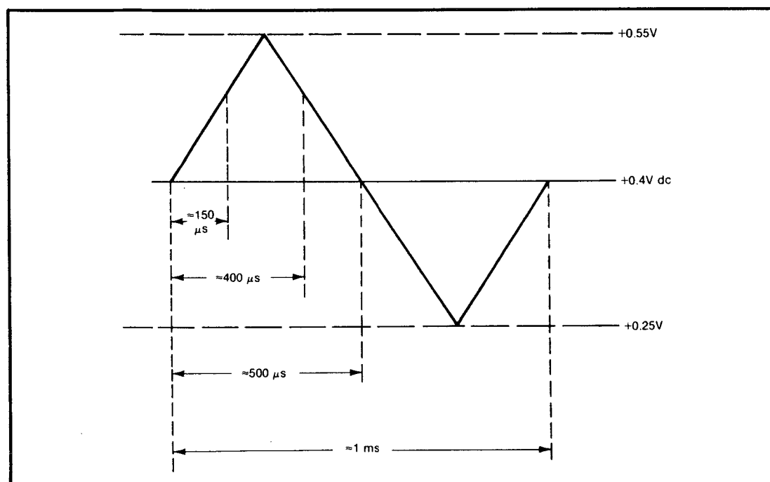
Figure 4-20. Test Waveform
