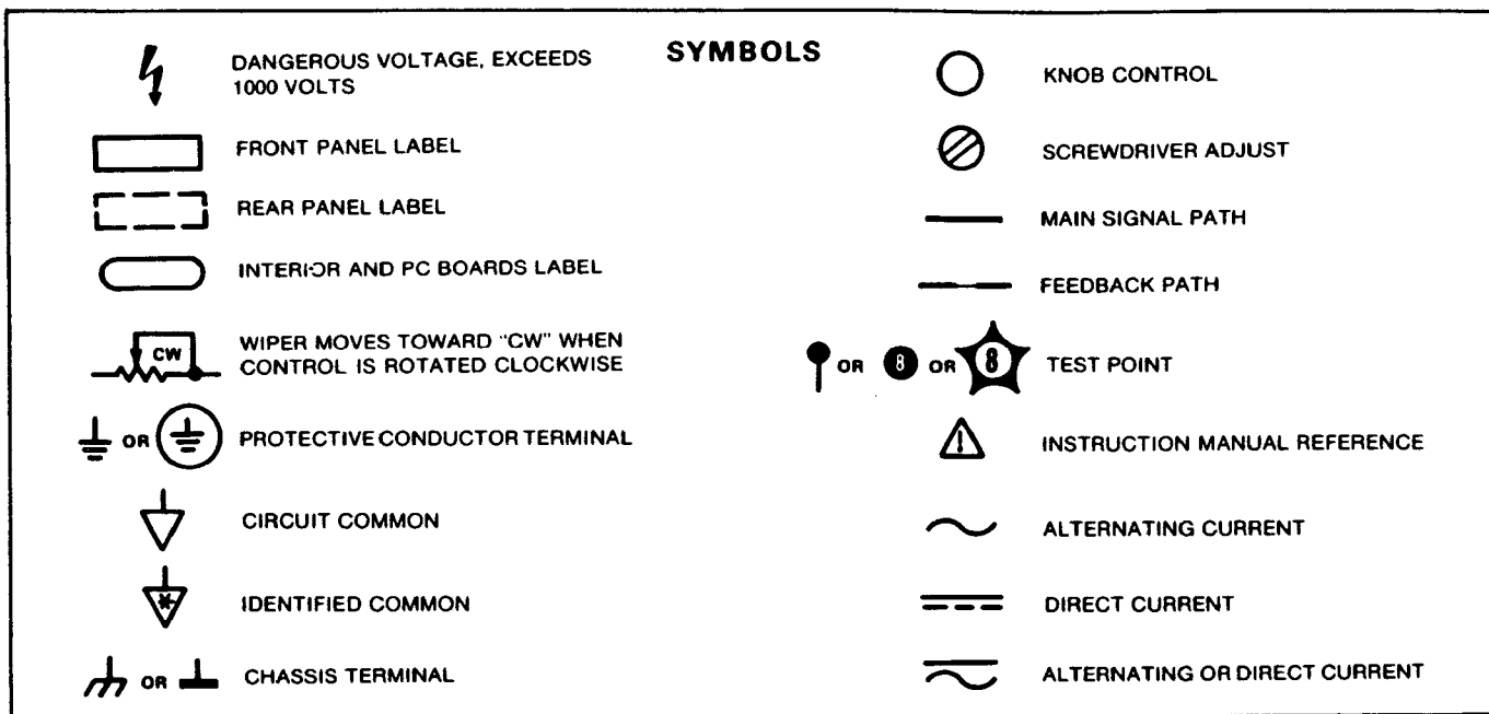
Figure 8-1. Schematic Diagram Symbols
