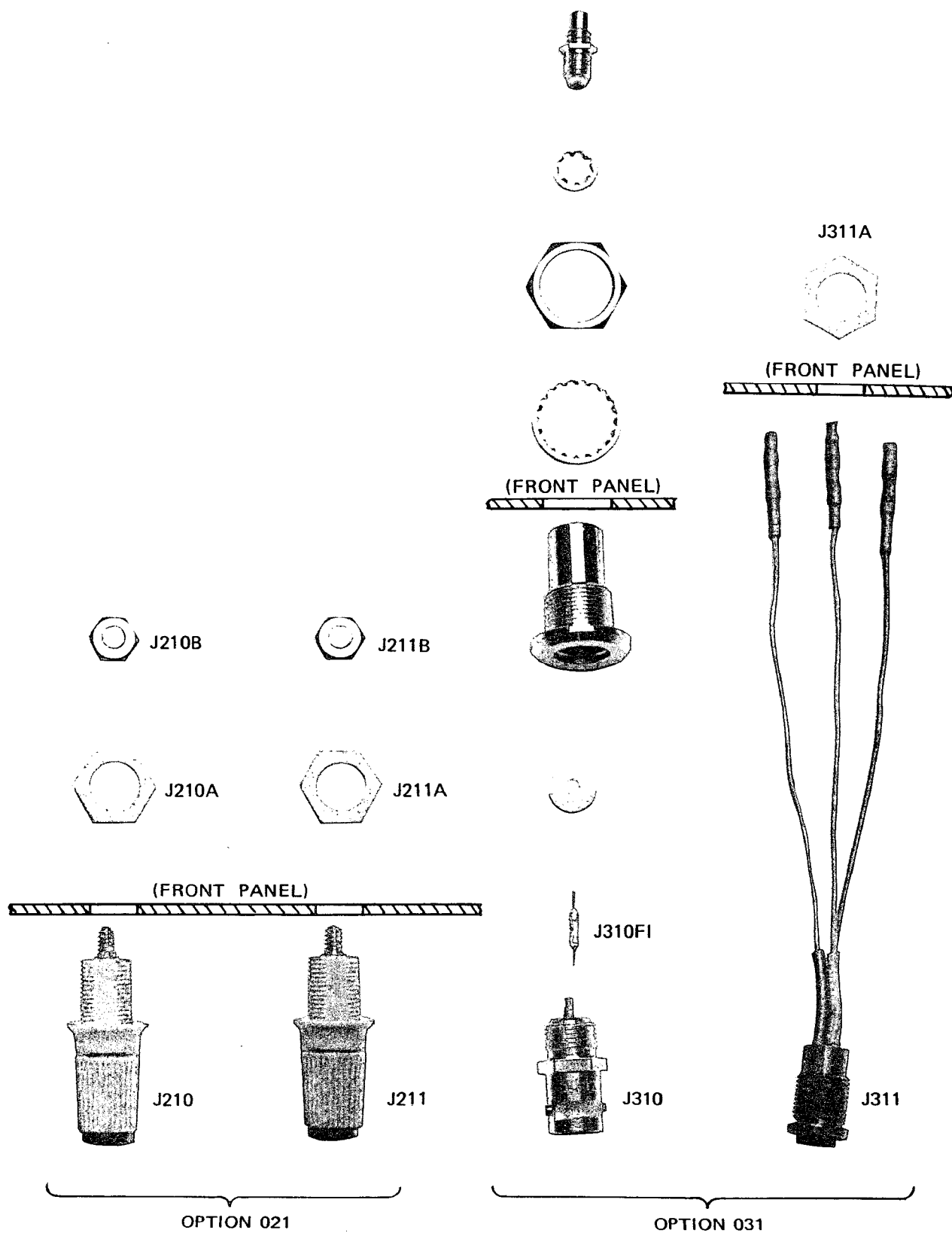
Figure 6-3. Option 050 (Options 021 & 031) Front Panel Hardware
