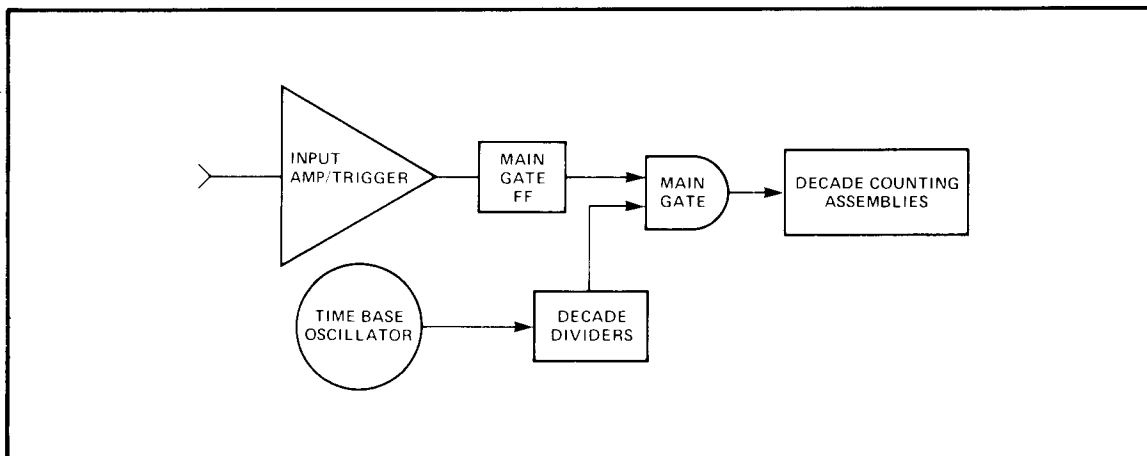
Figure 3-2. Measuring Period
