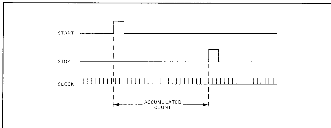
Figure 3-4. Clock Pulses
