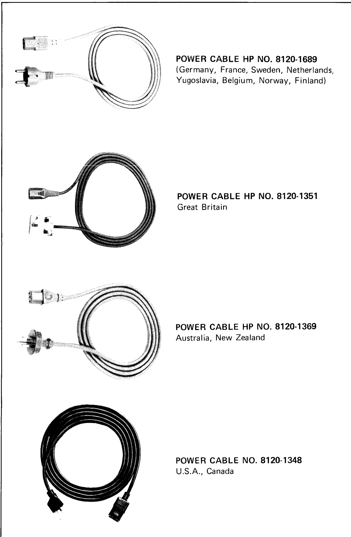
Figure 2-1. Power Cables
