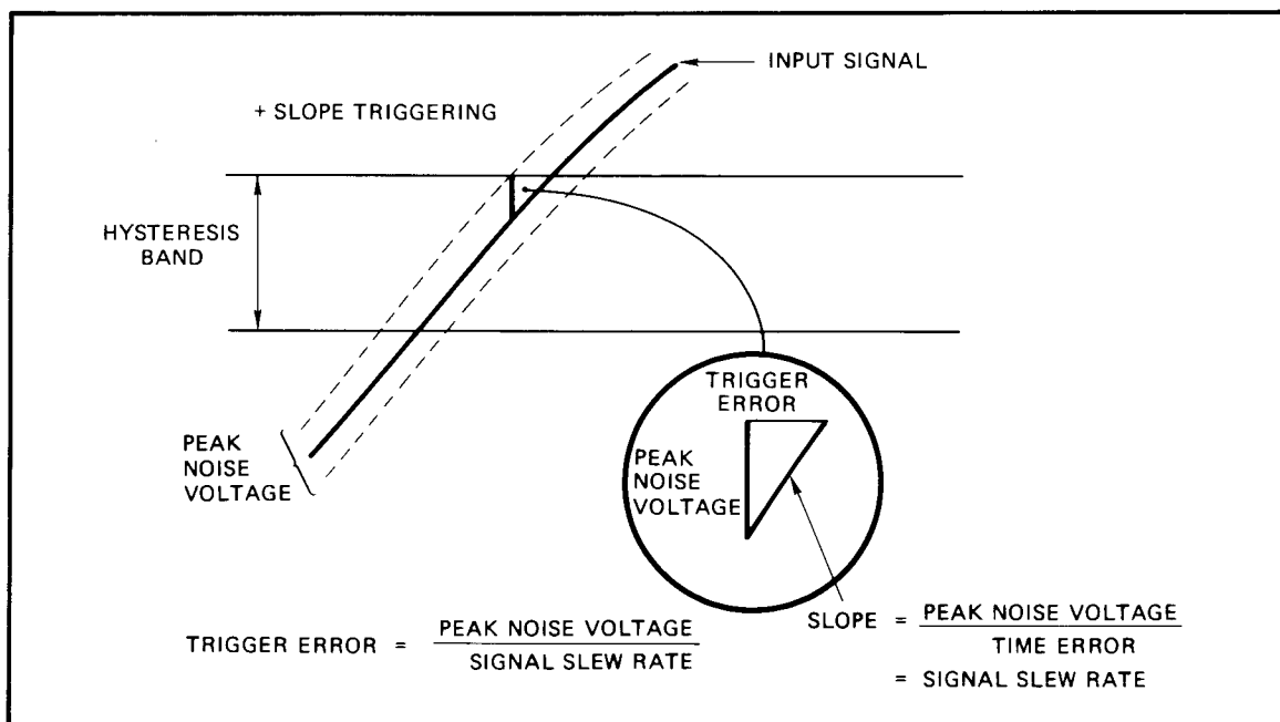
Figure 3-7. Trigger Error
