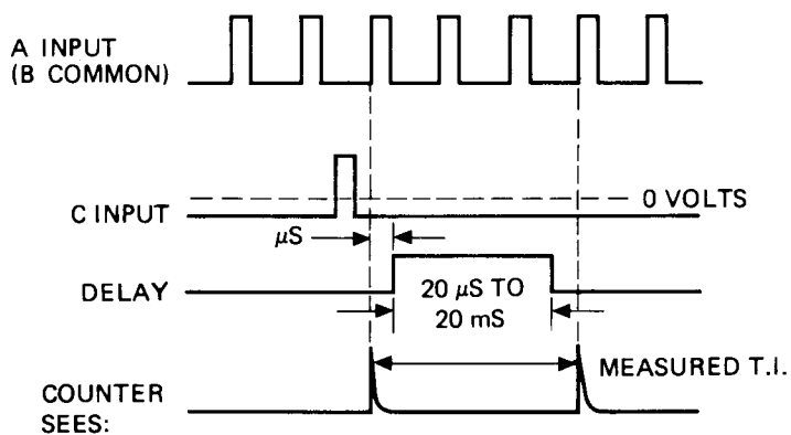
Figure 3-20. Time Interval Average Delay Mode
