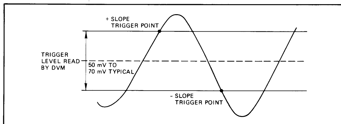
Figure 3-18. Hysteresis Band
