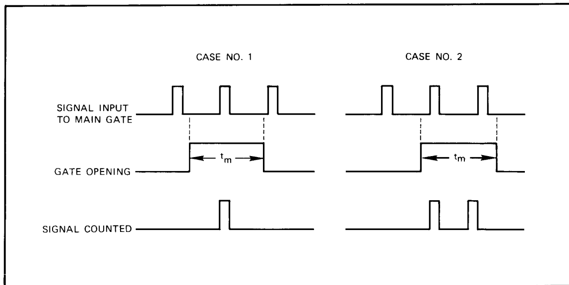
Figure 3-6. +1 Count Ambiguity
