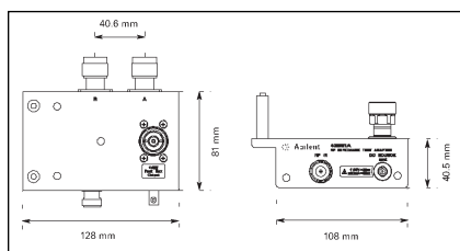
Agilent 43961A RF impedance test kit
