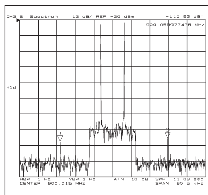
IMD measurement using list sweep function
