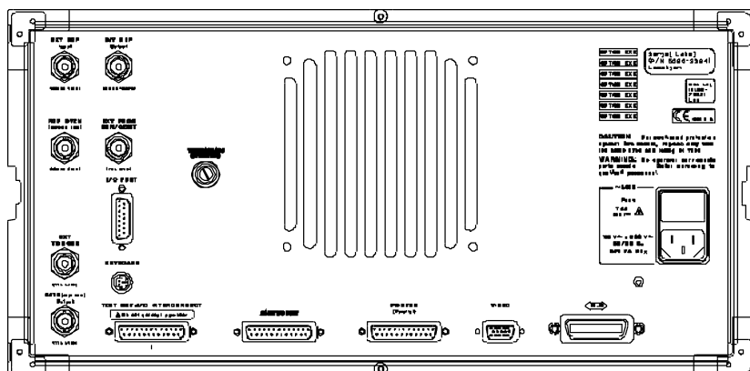
Agilent 4395A rear panel
