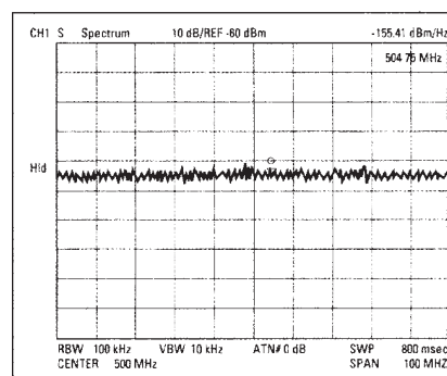
IMD measurement using list sweep function
