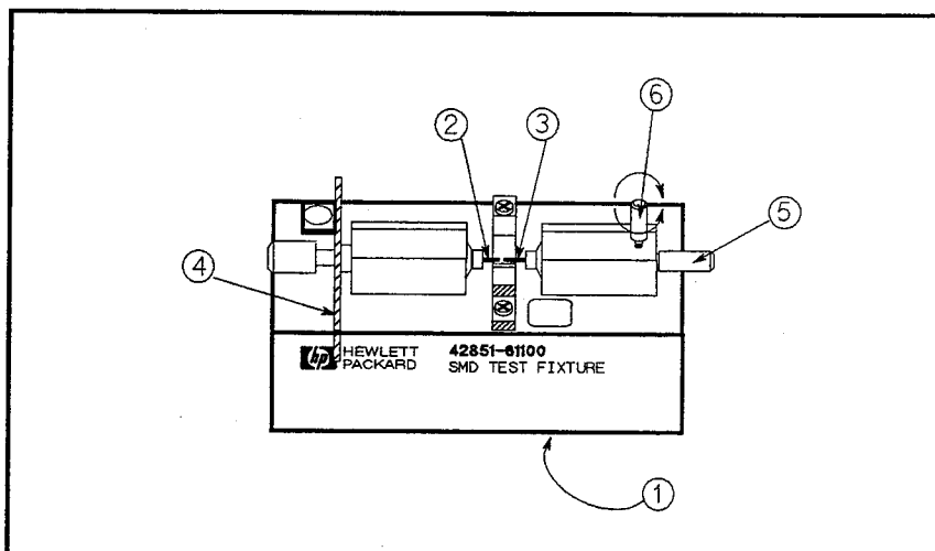
Figure 1-6. Overview of The SMD Test Fixture
