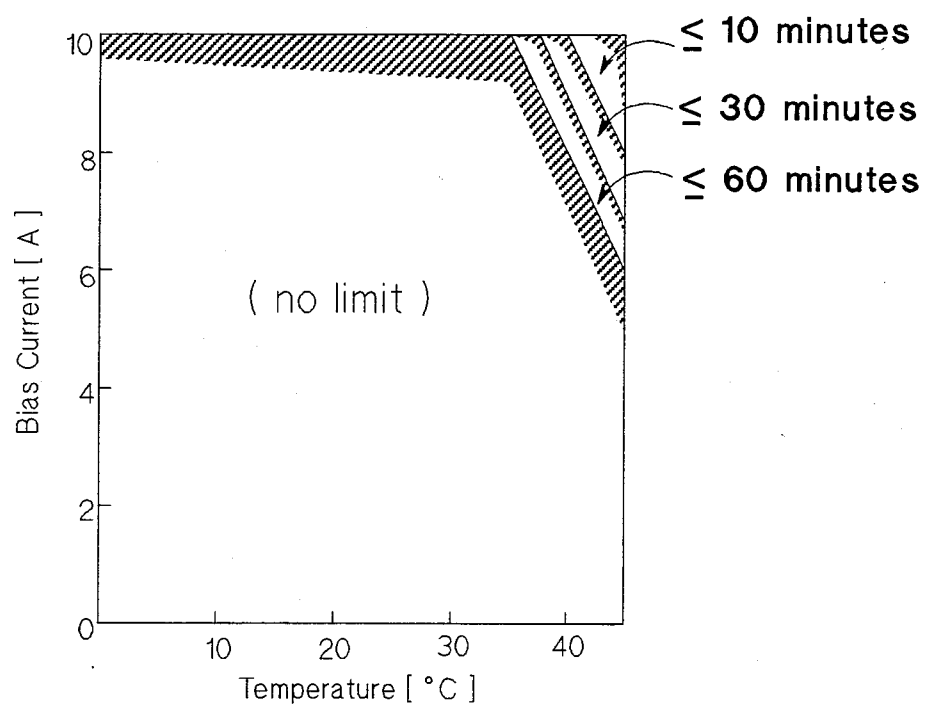
Figure 1-8. Maximum Continuous Running Time of the HP 42842C
