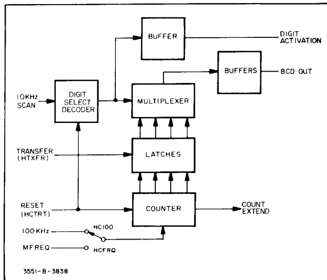
Figure 4-5. Data Accumulator.
