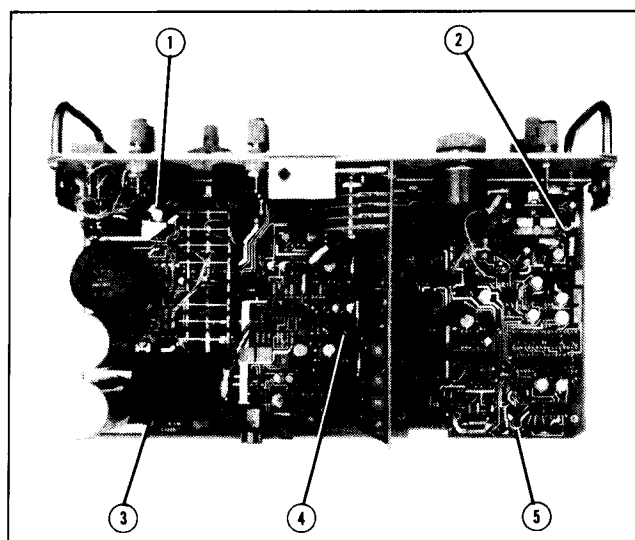
Figure 5-16. Shield Removal.
