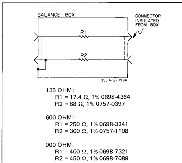
Figure 5-1. Impedance Box.
