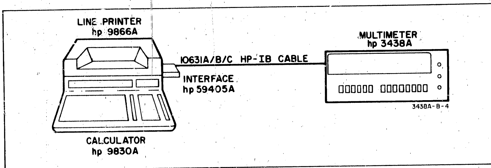
Figure 3-17. 9830A/HP-IB Application.
