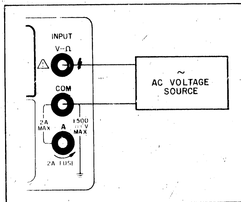
Figure 3-5. AC Voltage Measurement.
