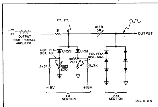
Figure 4-2. Sine Shaper.
