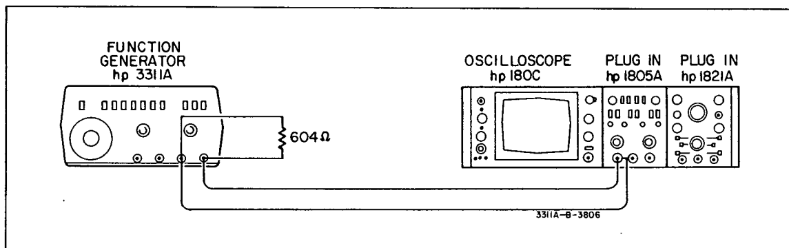
Figure 5-1. Amplitude Flatness.
