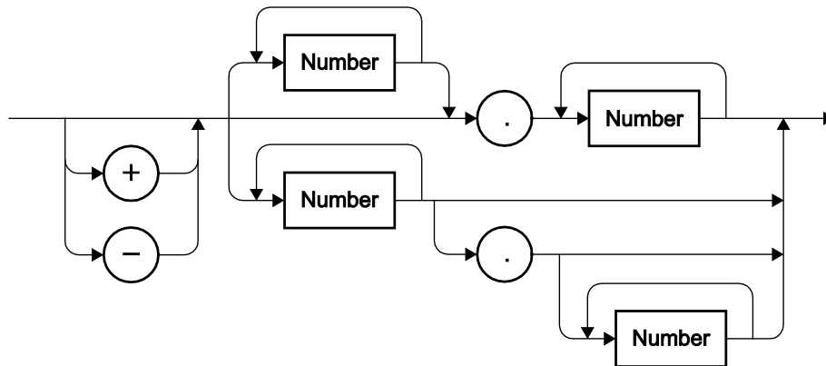
Figure 2.5. Mantissa Syntax
