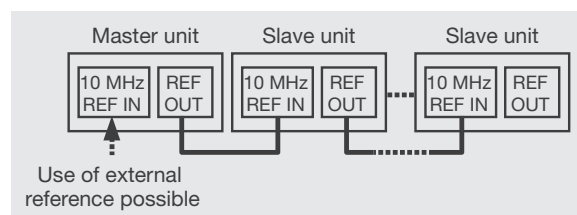
Connection method 2 (up to 4 units)
