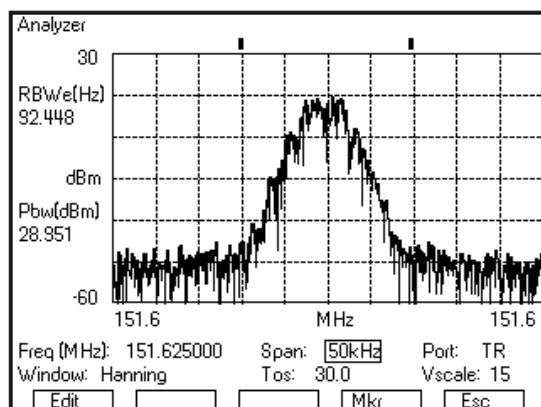
Full Screen Spectrum Analyzer
