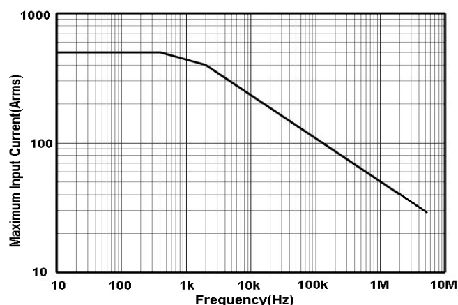
T3CP500-5 Continuous Maximum Current Input
