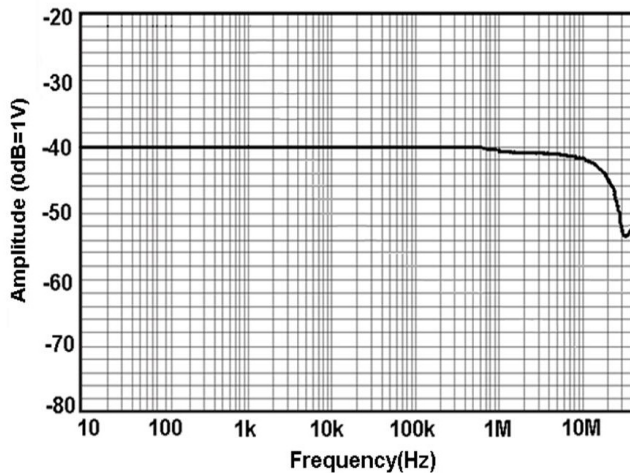
T3CP150-12 Frequency Response
