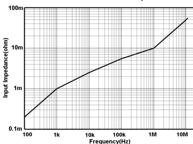
T3CP150-12 Insertion Impedance
