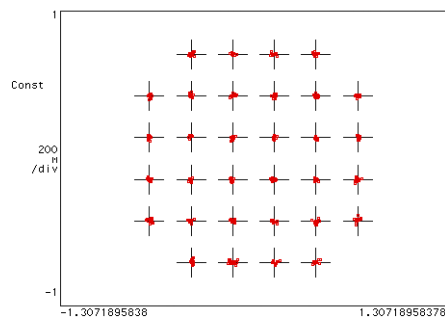
QAM32 constellation (5.8 GHz carrier)
