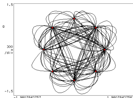
TETRA constellation (420 MHz carrier)
