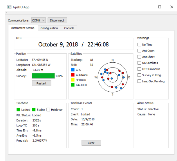
GNSSDO application
