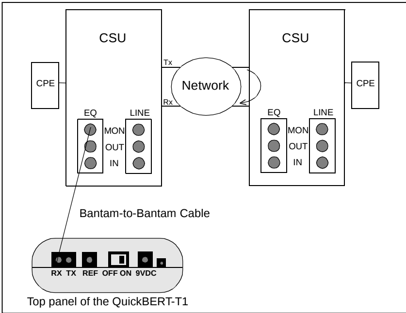
Figure 3-2. Capturing and Displaying DTMF Digits
