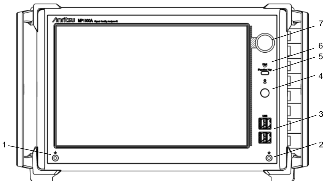
Figure 2.1-1 Front panel
