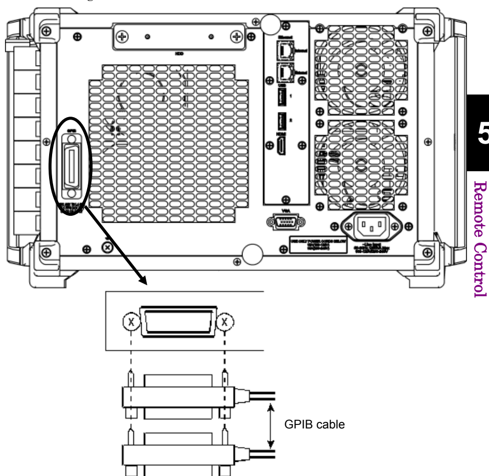
Figure 5.3-1 GPIB Cable Connection
