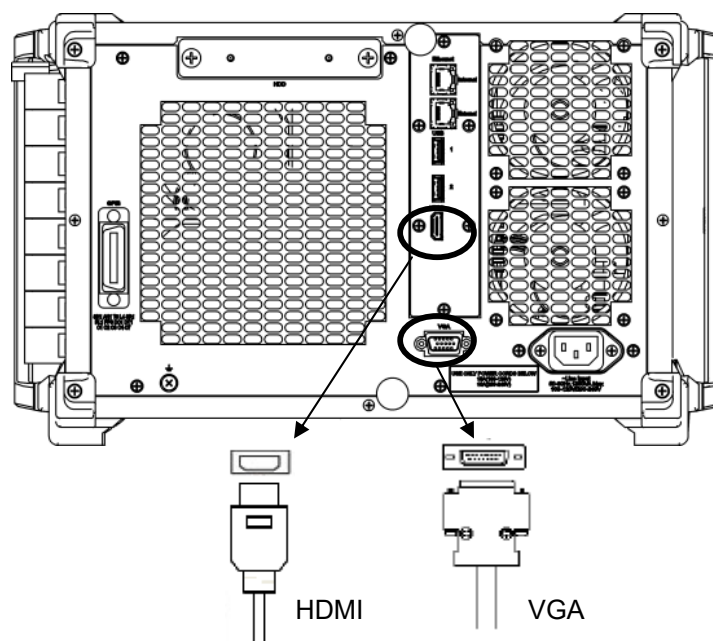
Figure 3.6-2 Display interface
