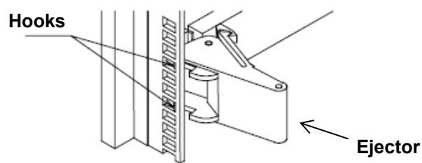
Figure 3.3.1-1 Module hooks
