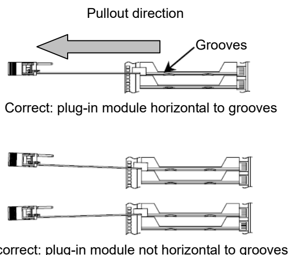
Figure 3.3.2-3 Module pullout
