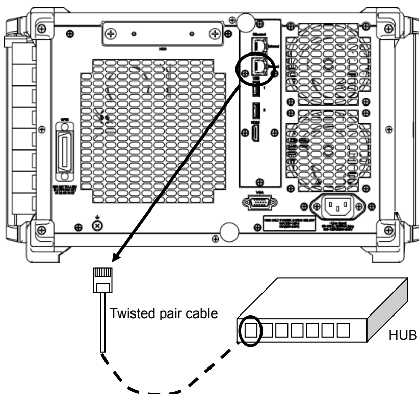
Figure 5.2-3 Ethernet Cable Connection
