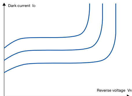
Temperature dependence of dark current-reverse voltage characteristic
