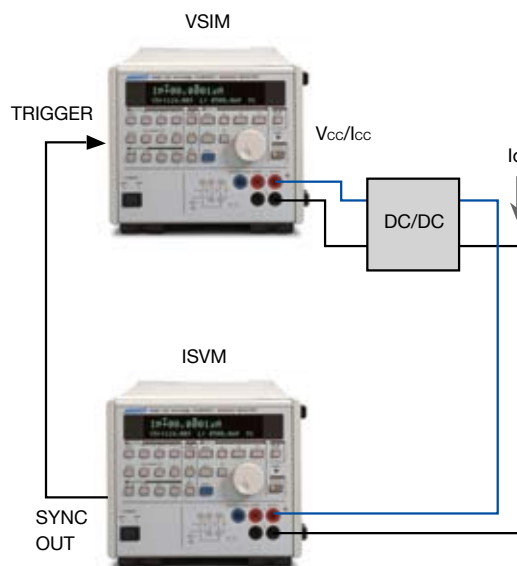
Parallel measurement of input current and output voltage
