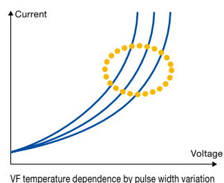
VF temperature dependence by pulse width variation
