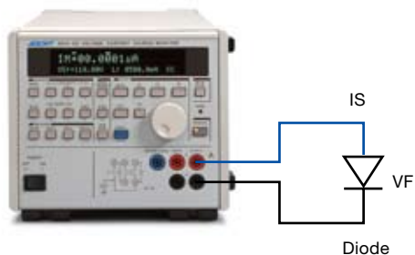
Current pulse sweep ISVM
