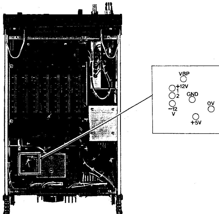
Figure 6 - 1 Supply Voltage Test Points
