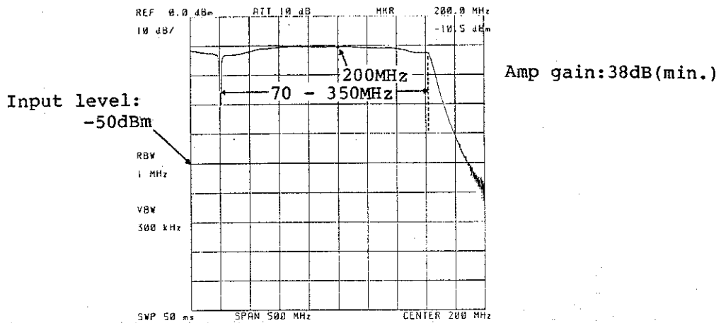
Figure 6 - 15 IF AMP Characteristics
