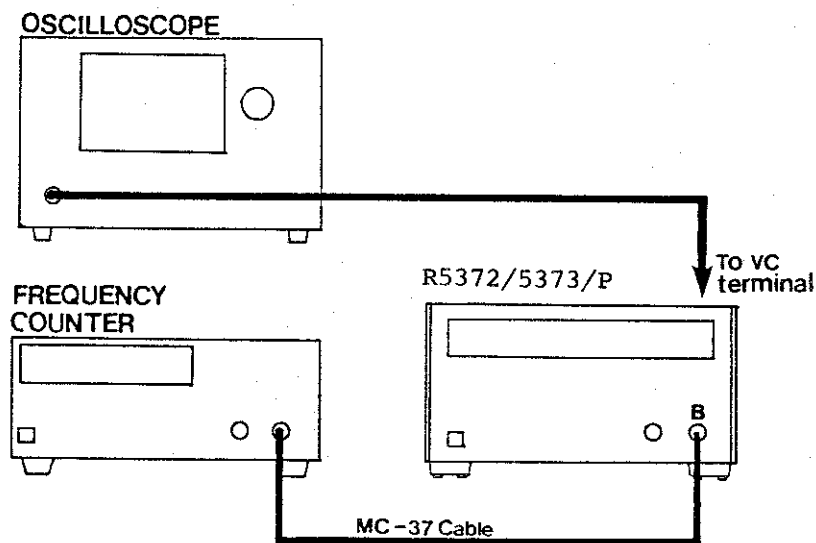
Figure 6 - 24 Setup for LOCK Check
