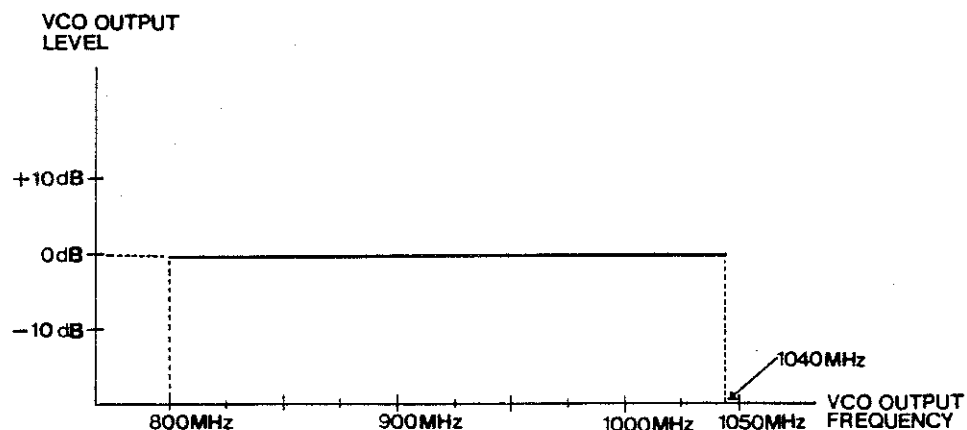
Figure 6 - 13 Relationships Between VCO Output Levels and Frequencies
