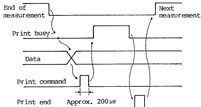
Figure 8 - 2 Timing Diagram of Data Output
