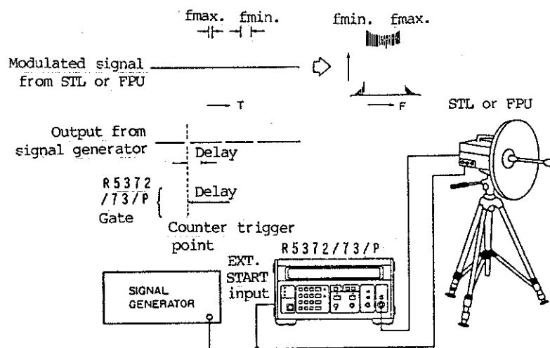
FM deviation quantity measurement example
