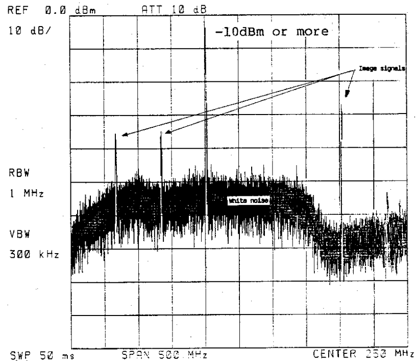
Figure 6 - 26 Output Level of IF AMP OUT Terminal
