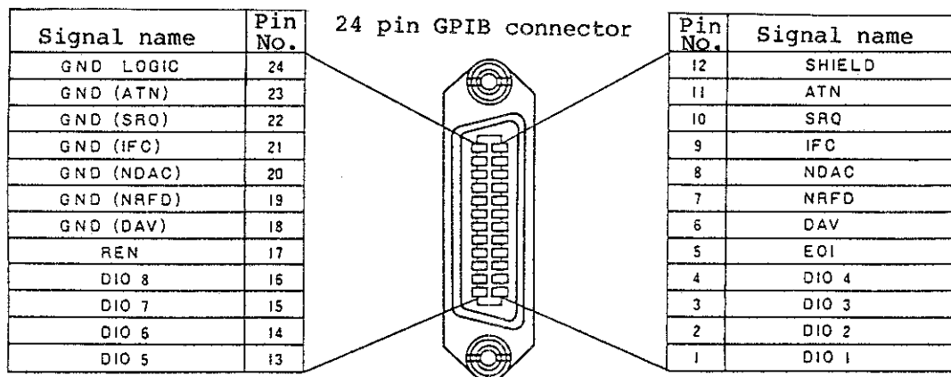
Figure 7 - 3 GPIB Connector Pin Assignment
