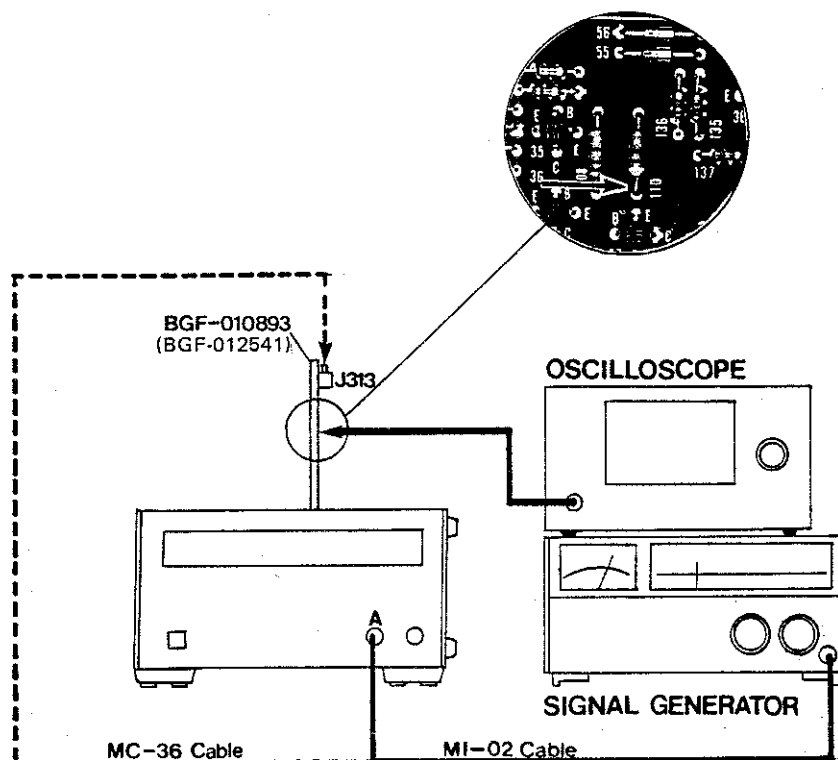
Figure 6 - 7 Setup for INPUT AMP & SCALER(BGF-010893) Adjustment
