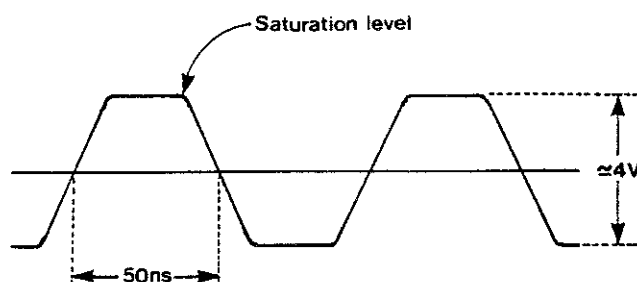
Figure 6 - 8 Waveforms for INPUT A AMP Offset Compensation
