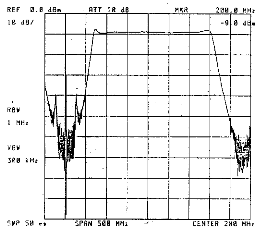
Figure 6 - 18 PREAMP characteristics (including the IF AMP and SAMPLER characteristics)
