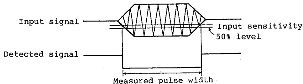
Figure 3 - 4 Modulated Pulse Width Measurement
