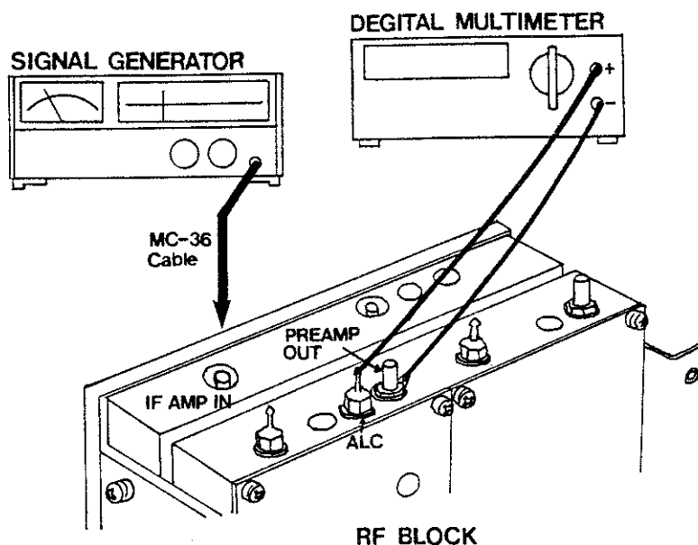
Figure 6 - 16 Setup for IF AMP Adjustment (2)
