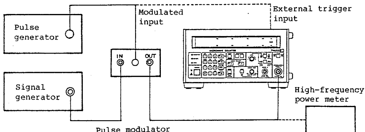
Figure 4 - 1 Instrument Connections for Burst Wave Carrier Frequency Measurement
