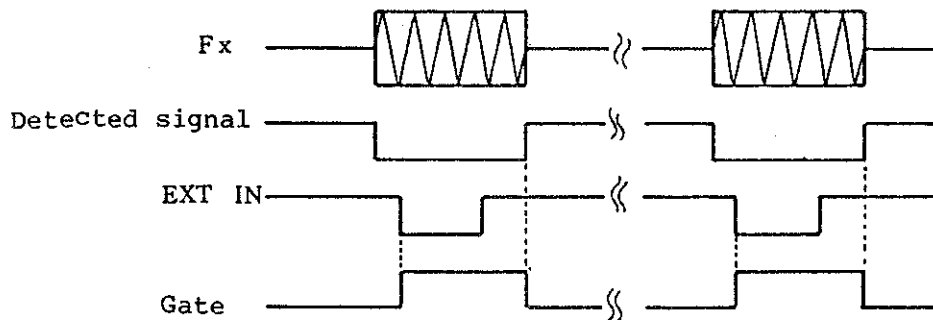
Figure 3 - 6 EXT START Mode
