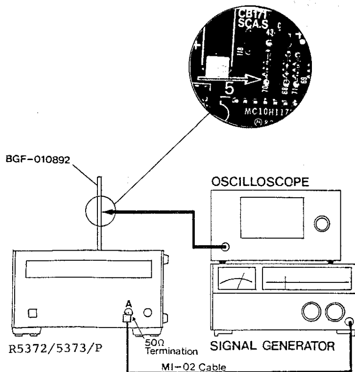
Figure 6 - 3 Setup for LOW F AMP Adjustment
