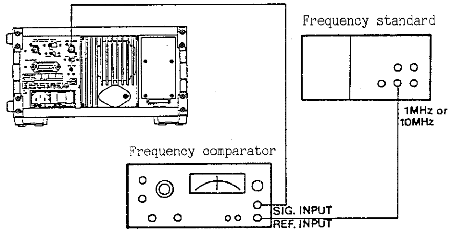
Figure 5 - 1 Calibration using frequency standard
