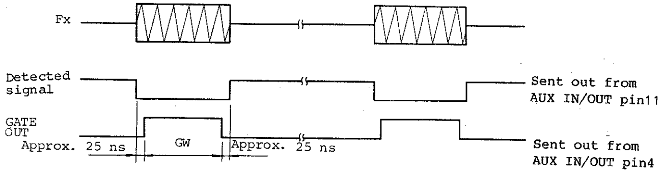
Figure 3 - 4 (b) Burst Wave Measurement on R5372P/5373P
