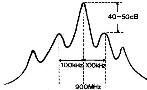
Figure 6 - 21 PLL Operation and Its Spurious Response Characteristics
