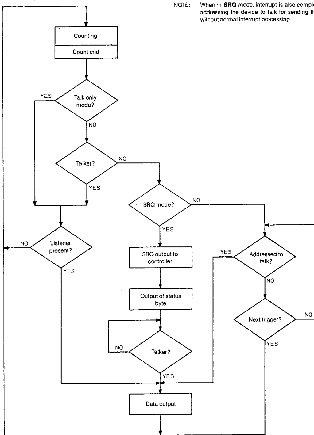
Figure 7 - 6 General Operation Flowchart
