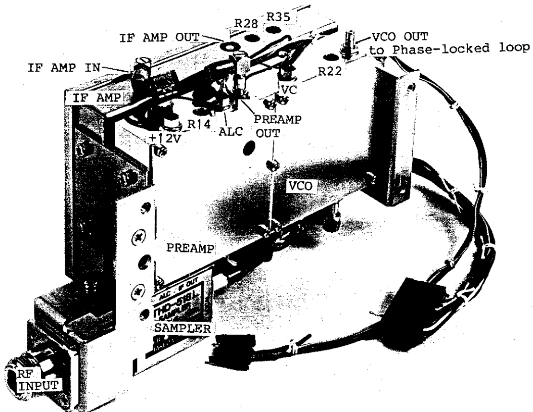
Figure 6 - 9 RF Block Assembly (controls and terminals location)
