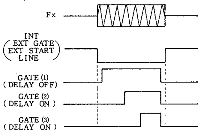
Figure 3 - 7 DELAYED GATE Mode
