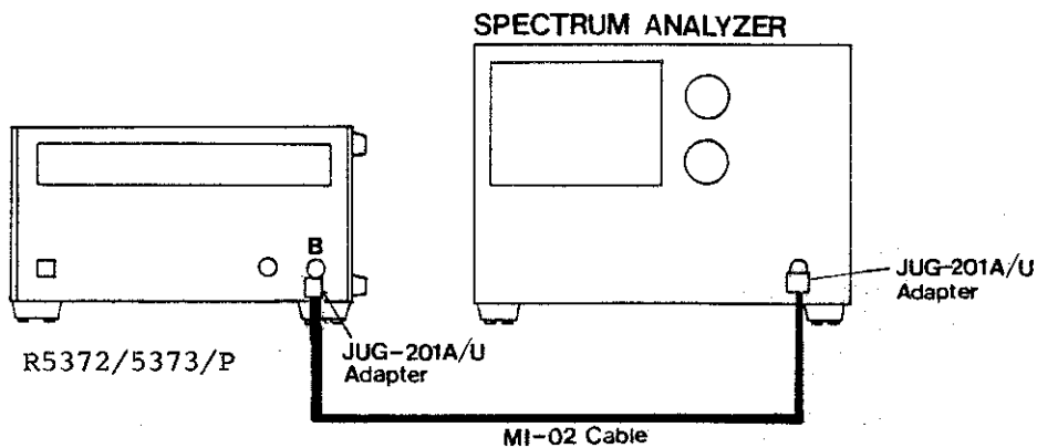
Figure 6 - 19 Setup for PLL operation check
