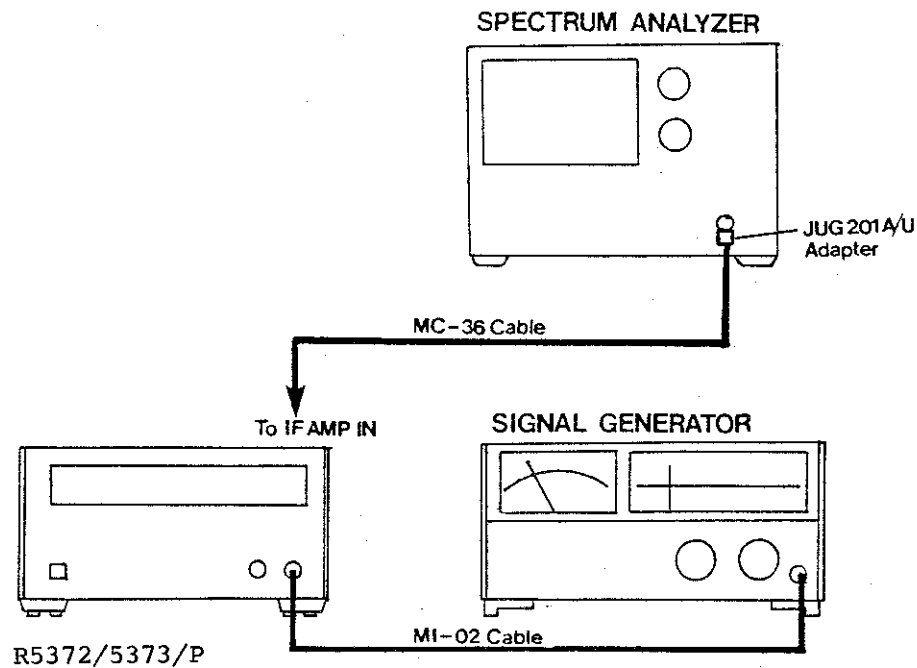
Figure 6 - 25. RF Section Test Setup
