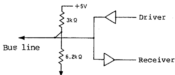
Figure 7 - 2 Signal Line Termination
