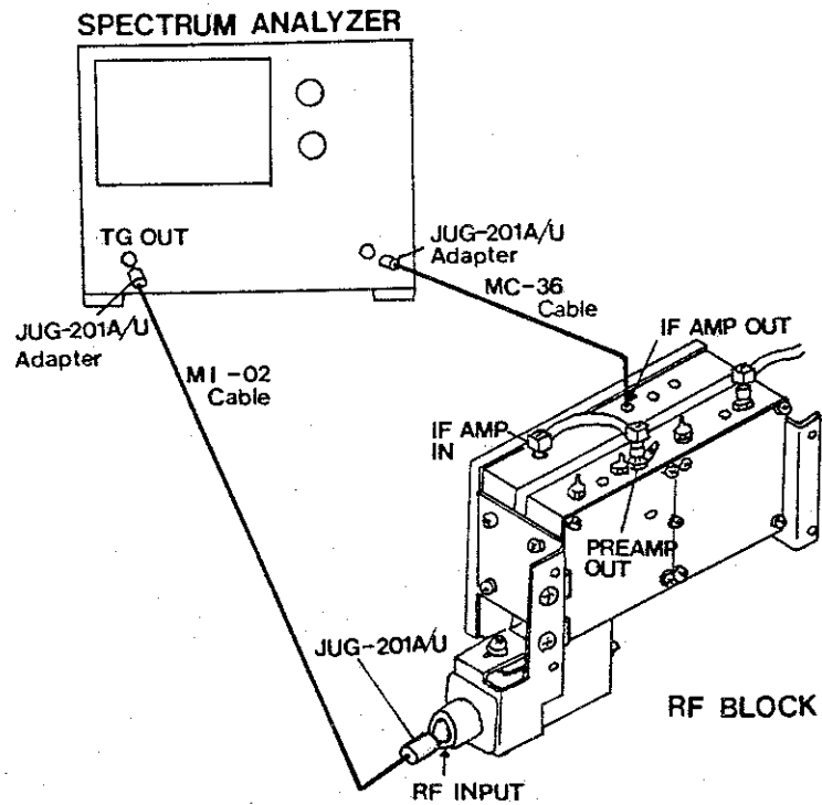
Figure 6 - 17 Setup for PREAMP adjustment
