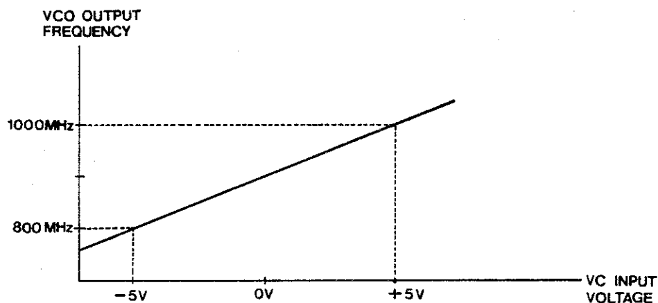
Figure 6 - 12 Relationships Between VC Input Voltage Values and VCO Output Frequencies
