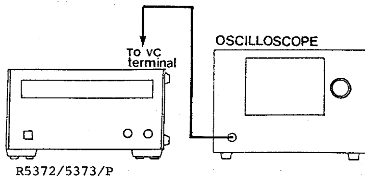
Figure 6 - 22 Setup for LIMITER check
