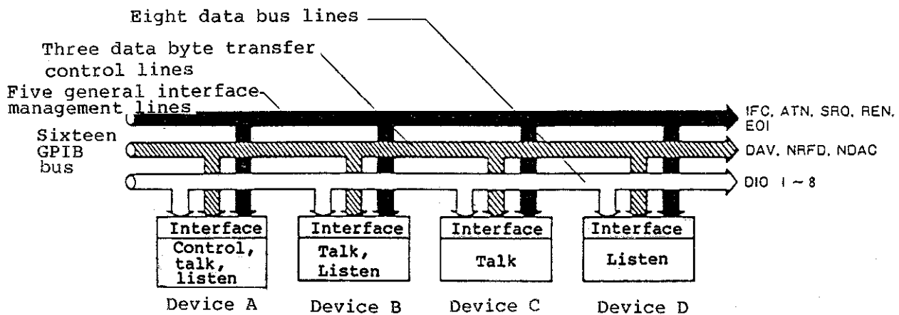
Figure 7 - 1 General Structure of GPIB
