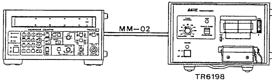
Figure 8 - 1 Connection to TR6198
