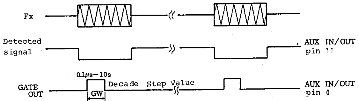
Figure 3 - 3 (a) Burst Wave Measurement on R5372/5373
