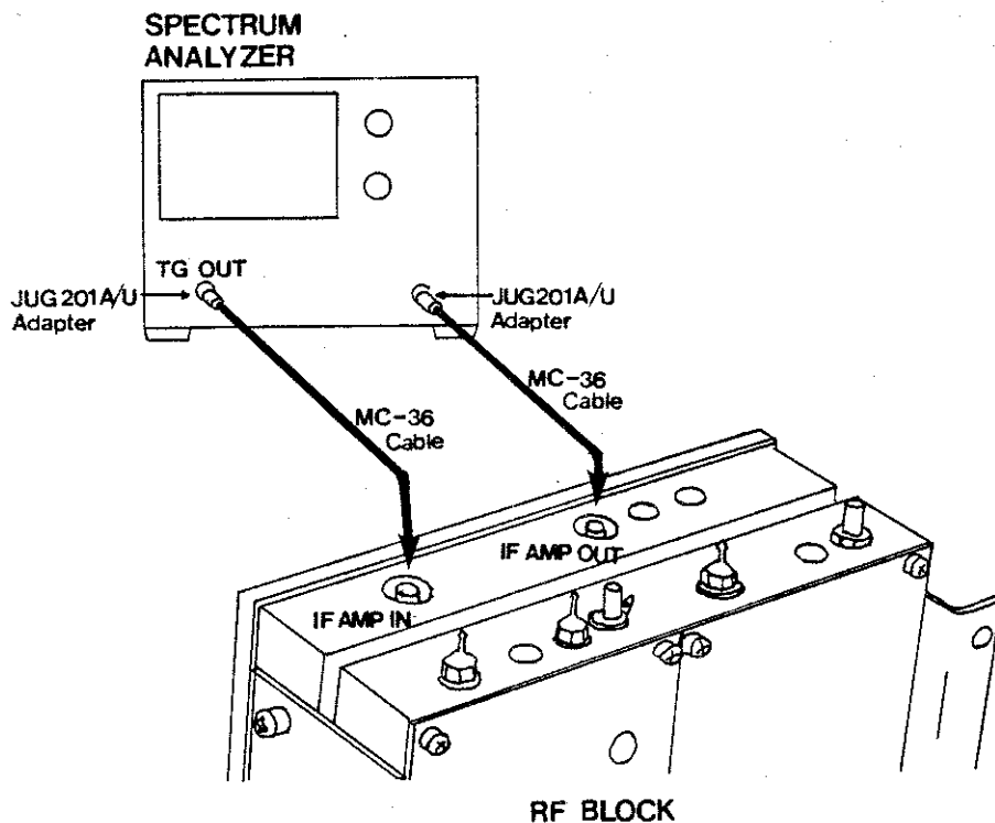
Figure 6 - 14 Setup for IF AMP Adjustment (1)
