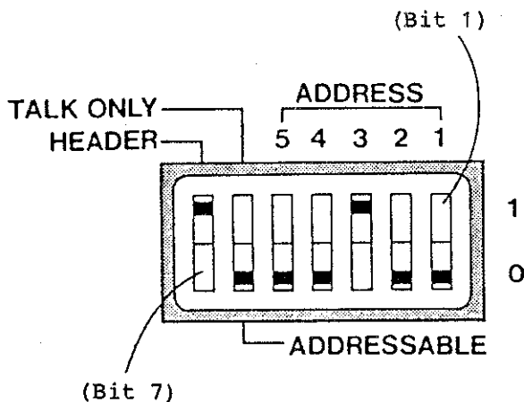
Figure 7 - 5 ADDRESS Switch
