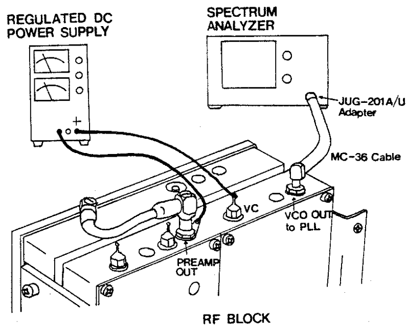
Figure 6 - 11 Setup for VCO Adjustment
