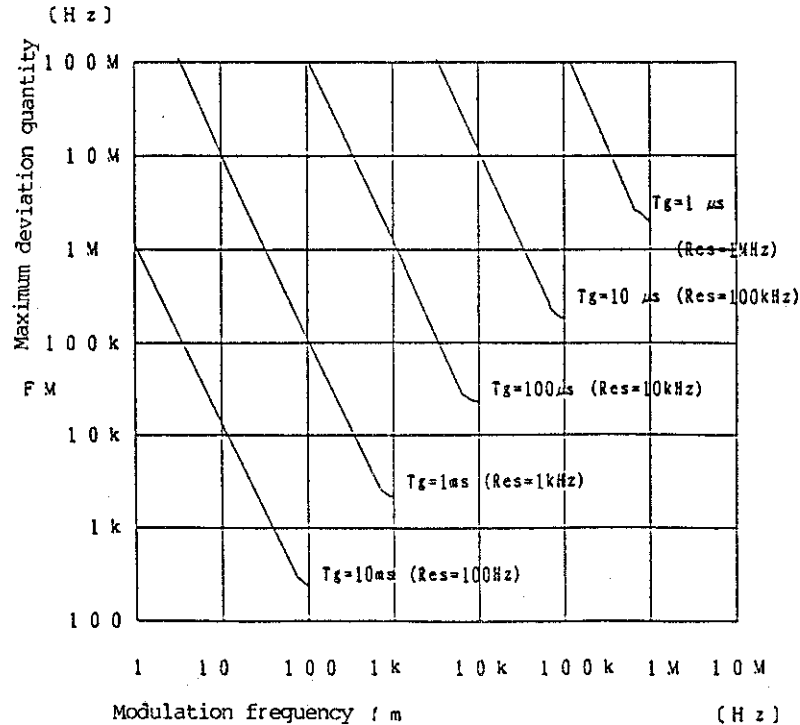
Figure 3 - 9 The Optimum GATE Time for FM Deviation
