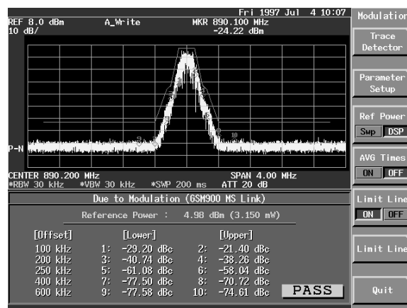
▲ Modulation spectrum measurement
