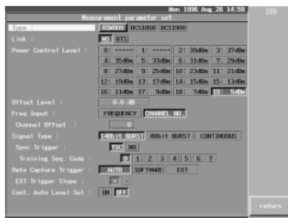
▲ GSM setting screen
