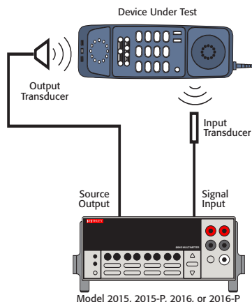
Figure 2. Total Harmonic Distortion Analysis and Frequency Response of a Portable Wireless Telecommunication Device
