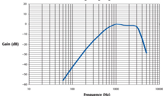
C-Message Weighting Filter
