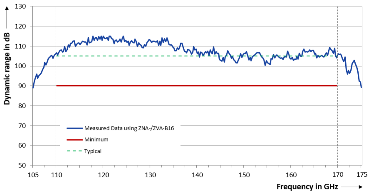
Dynamic range versus frequency of the R&S®ZC170
