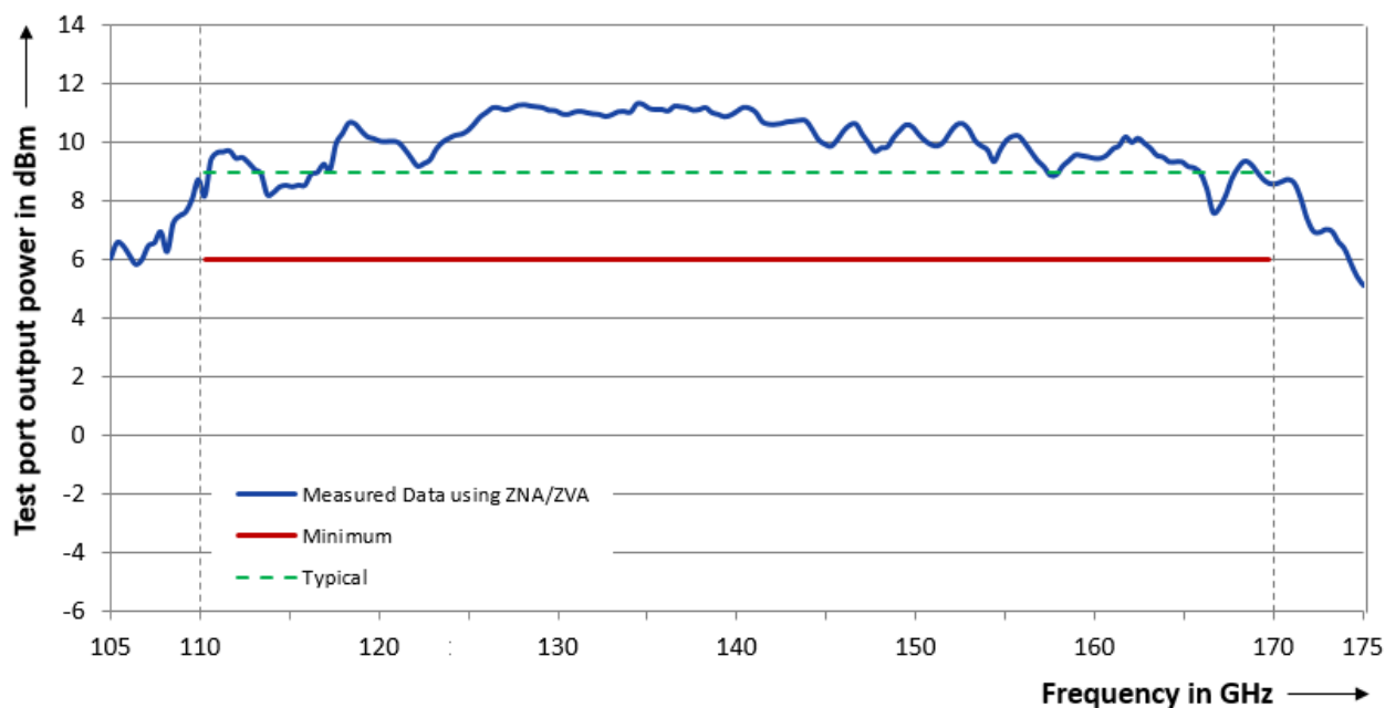
Test port output power versus frequency of the R&S®ZC170
