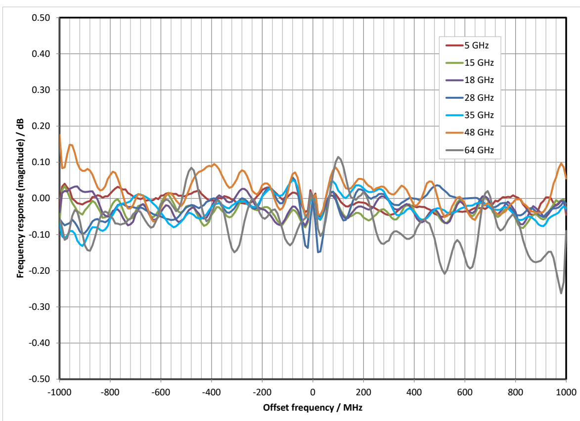
Measured RF modulation frequency response (magnitude) with internal baseband I/Q, wideband baseband
