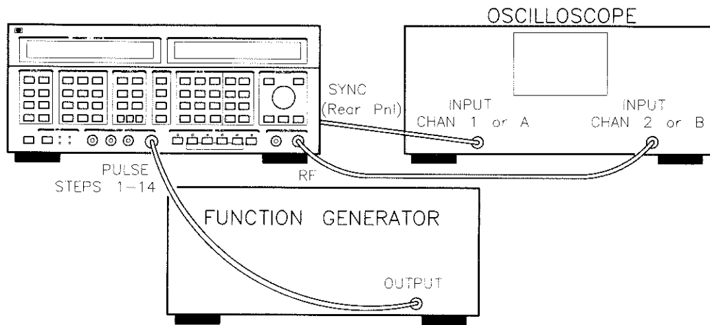
Figure 2-12. Equipment Setup for Pulse Modulation Procedure #2.
