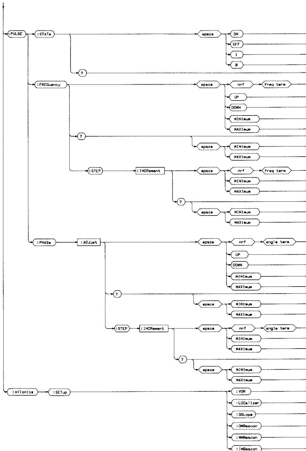
Figure E-12. LF Source Subsystem. (6 of 6)
