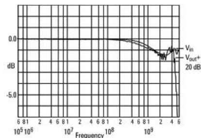
Figure 3.11. Notice how closely output matches input. Graph shows V_{in} and V_{out} when driven from a 25 \Omega source.
