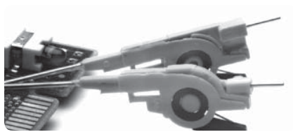
Figure 9.2. Extremely small-sized clips for probing PQFP and SOIC SMT packages.
