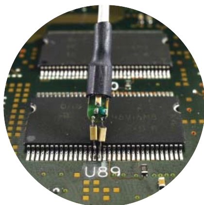
Figure 3.1. Agilent 1130A/31A/32A/34A InfiniiMax high-performance active probe.
