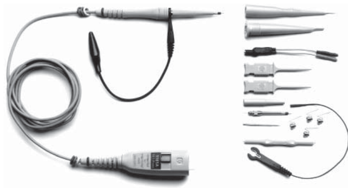
Figure 2.5. Agilent 116XA family general purpose replacement probes.
